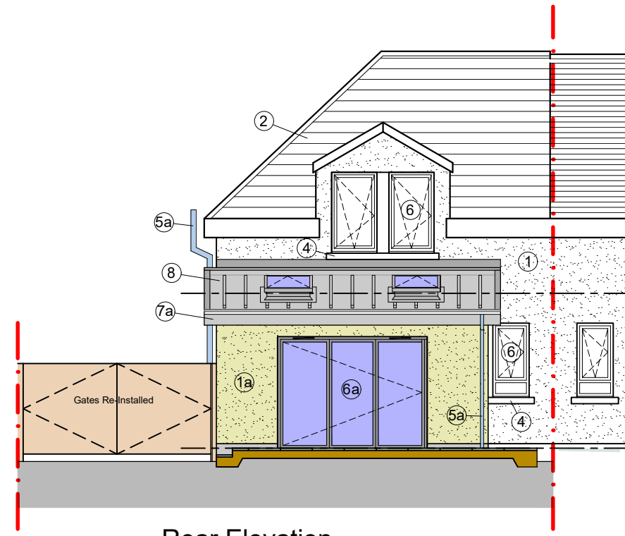
Rear Elevation
