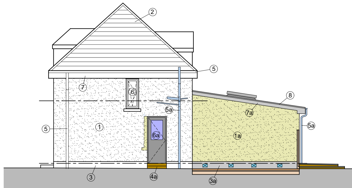
Gable Elevation
