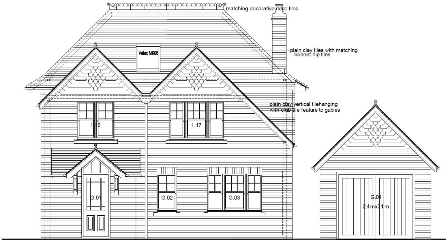
NORTH WEST FRONT ELEVATION
