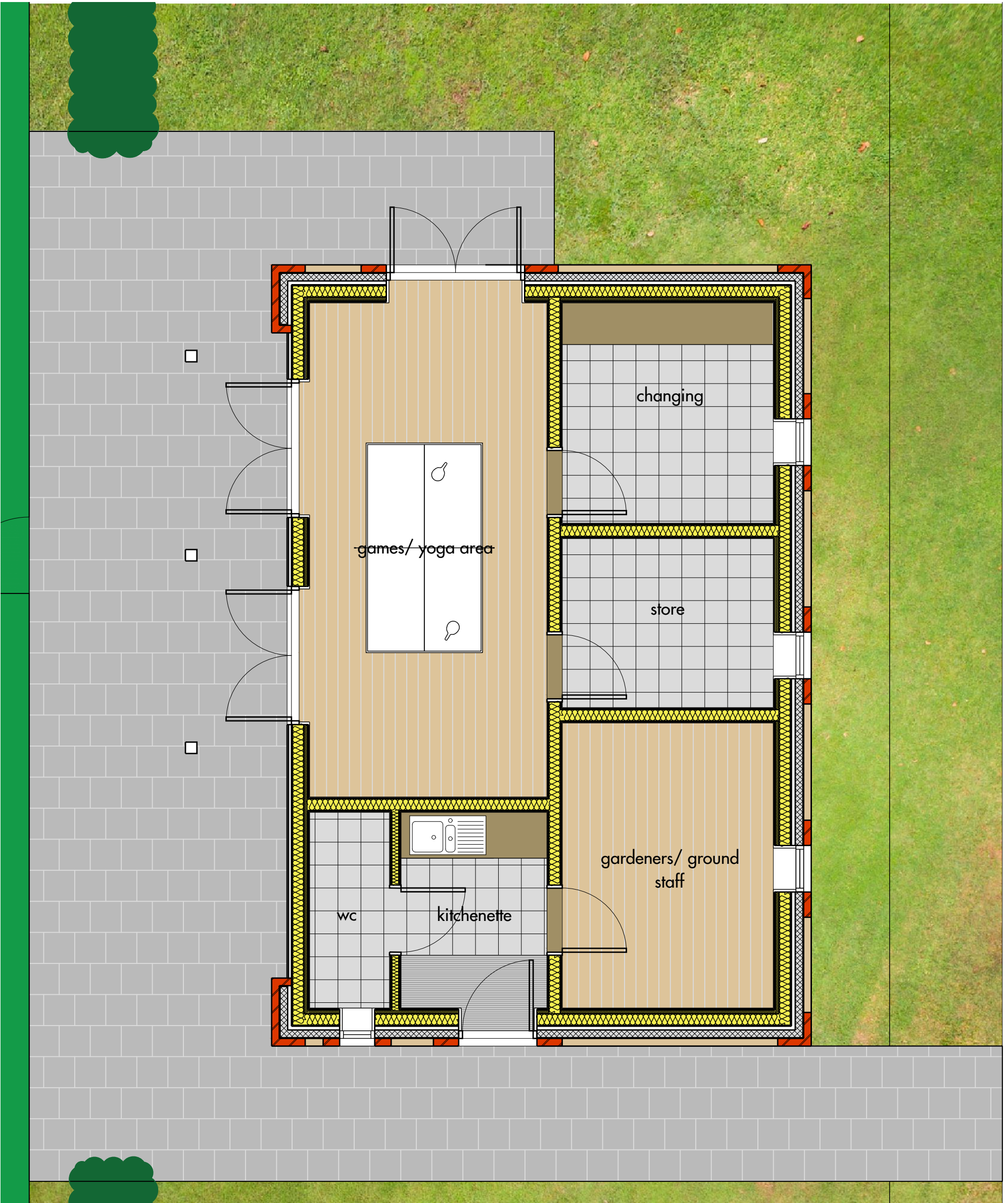
Floor plan
