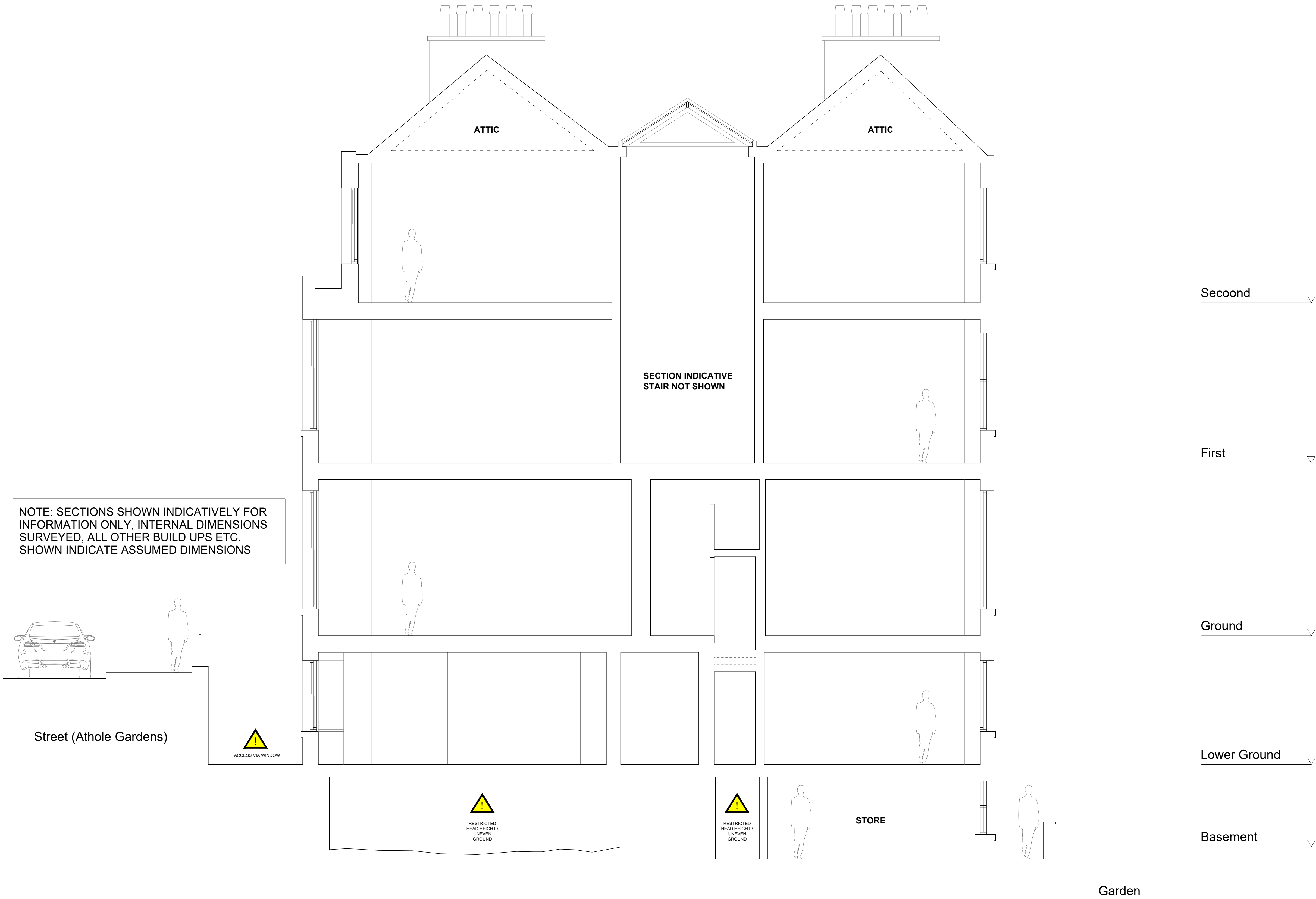
SECTION A - A
