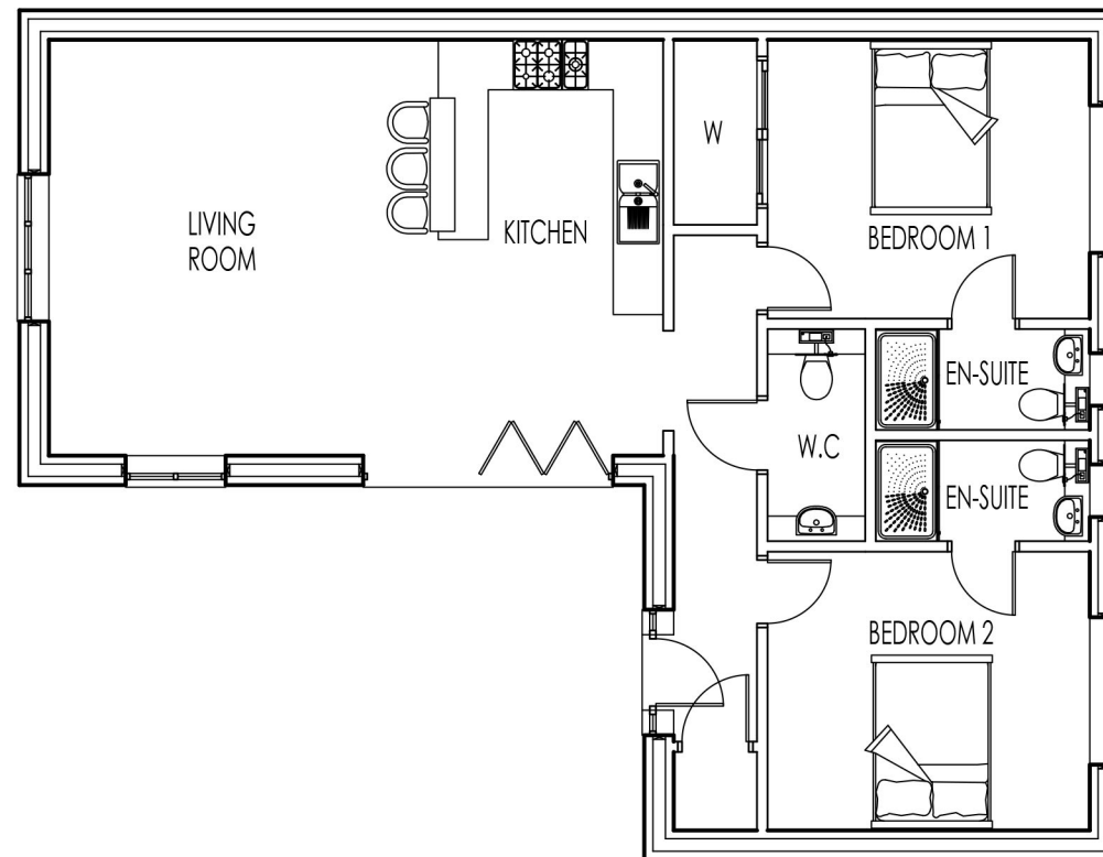
FLOOR PLANS
