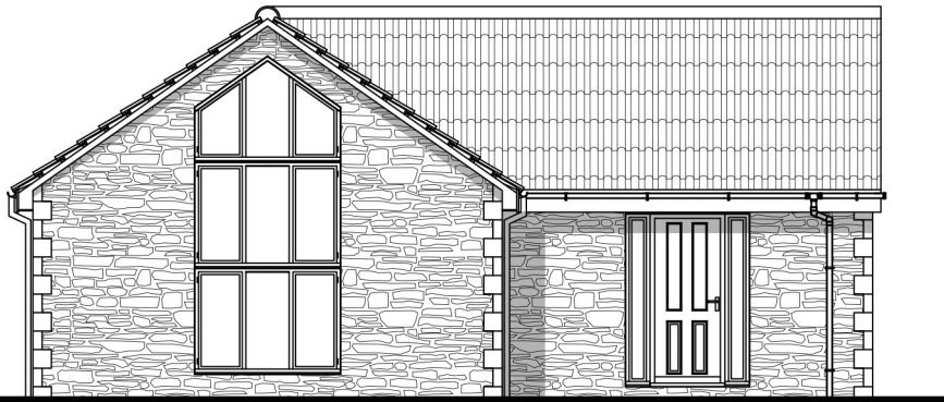
ELEVATION D
