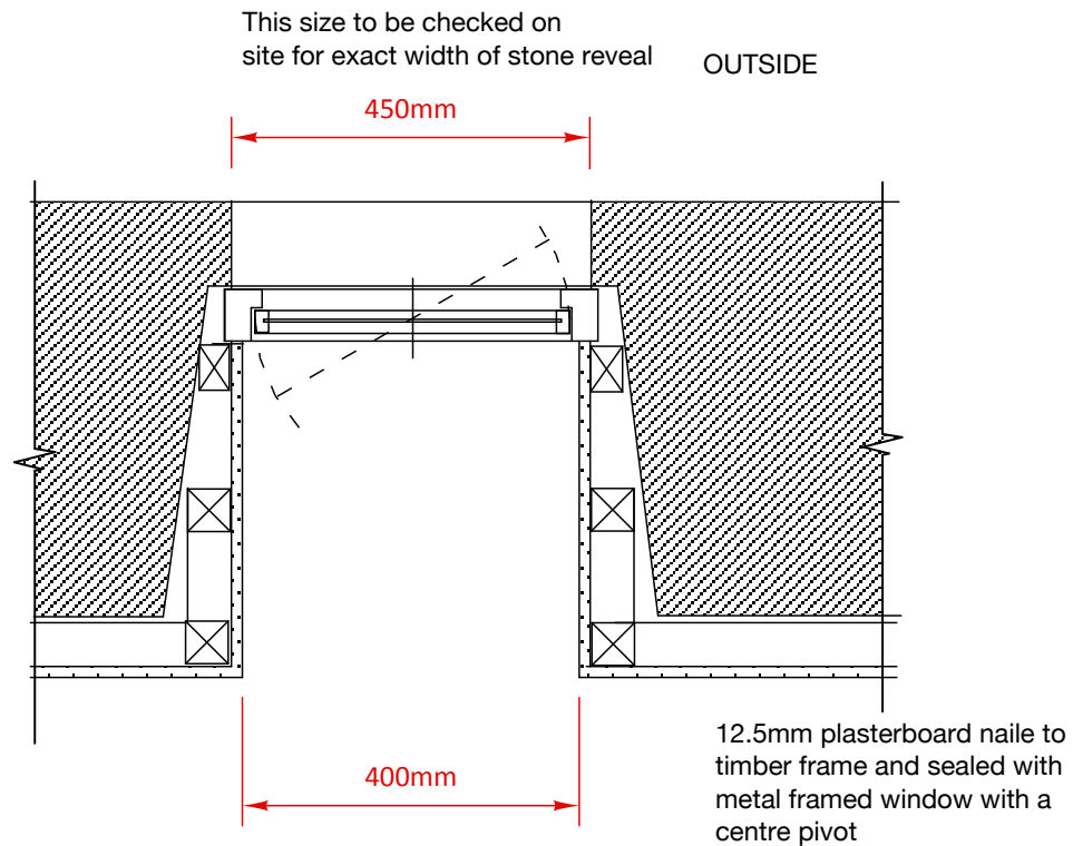
EXISTING WINDOW WITH CENTRE PIVOT...
