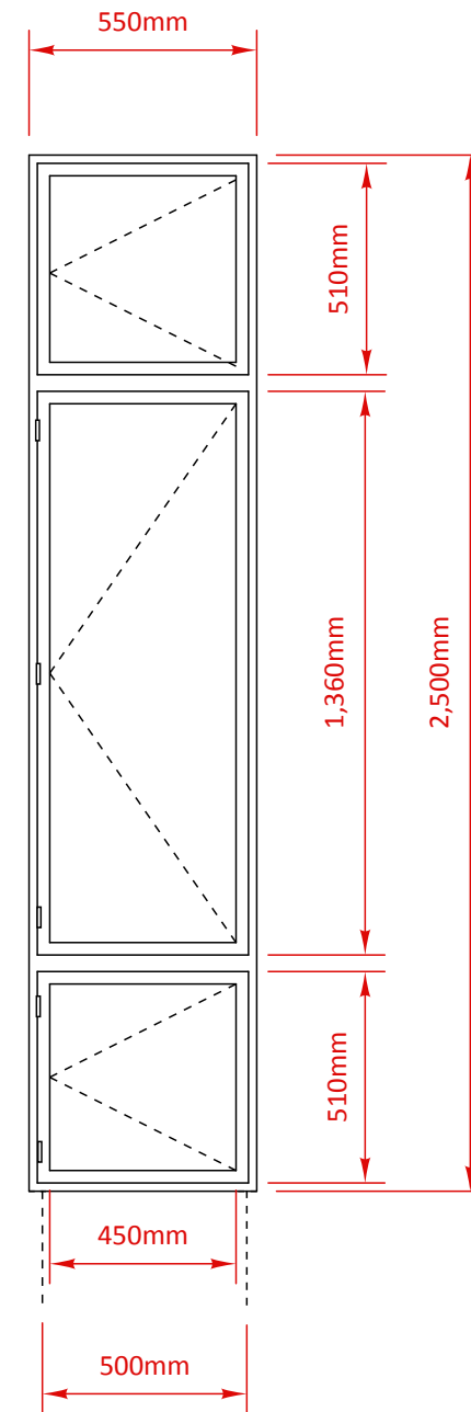
ELEVATION TO NEW WINDOW...
