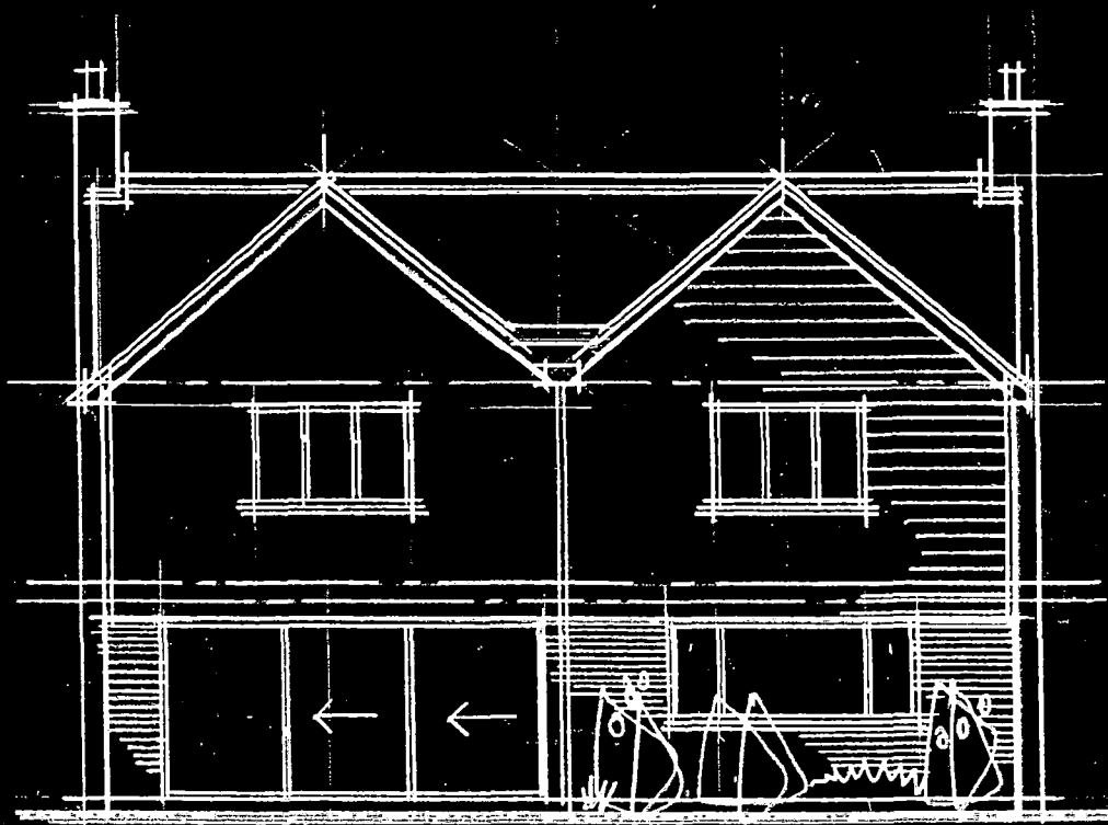
REAR ELEVATION (EAST)
