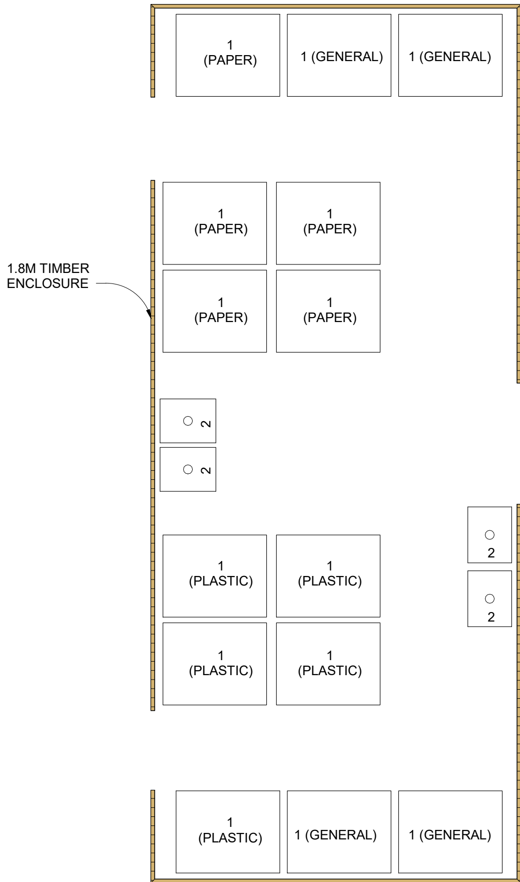
GROUND FLOOR
