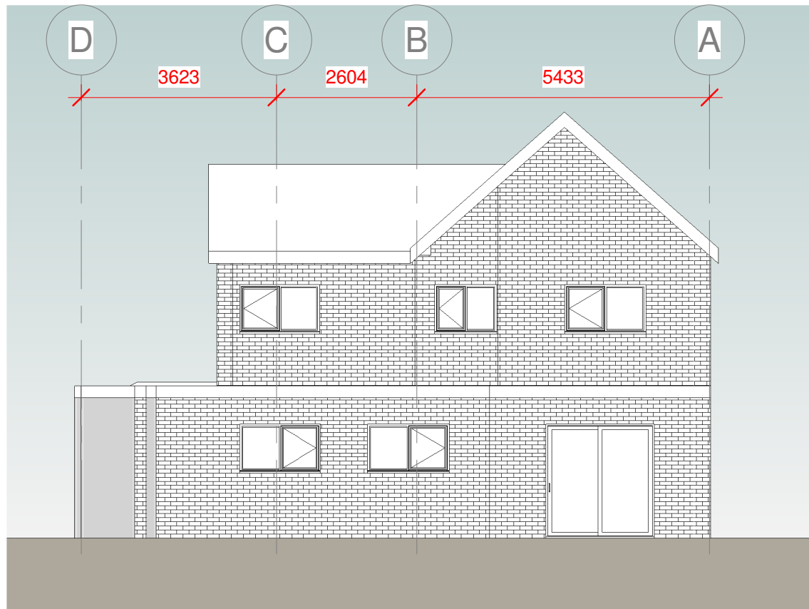
1 Existing Rear Elevation 1 : 100
