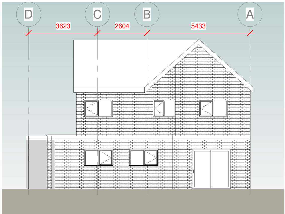
2 Proposed Rear Elevation 1 : 100
