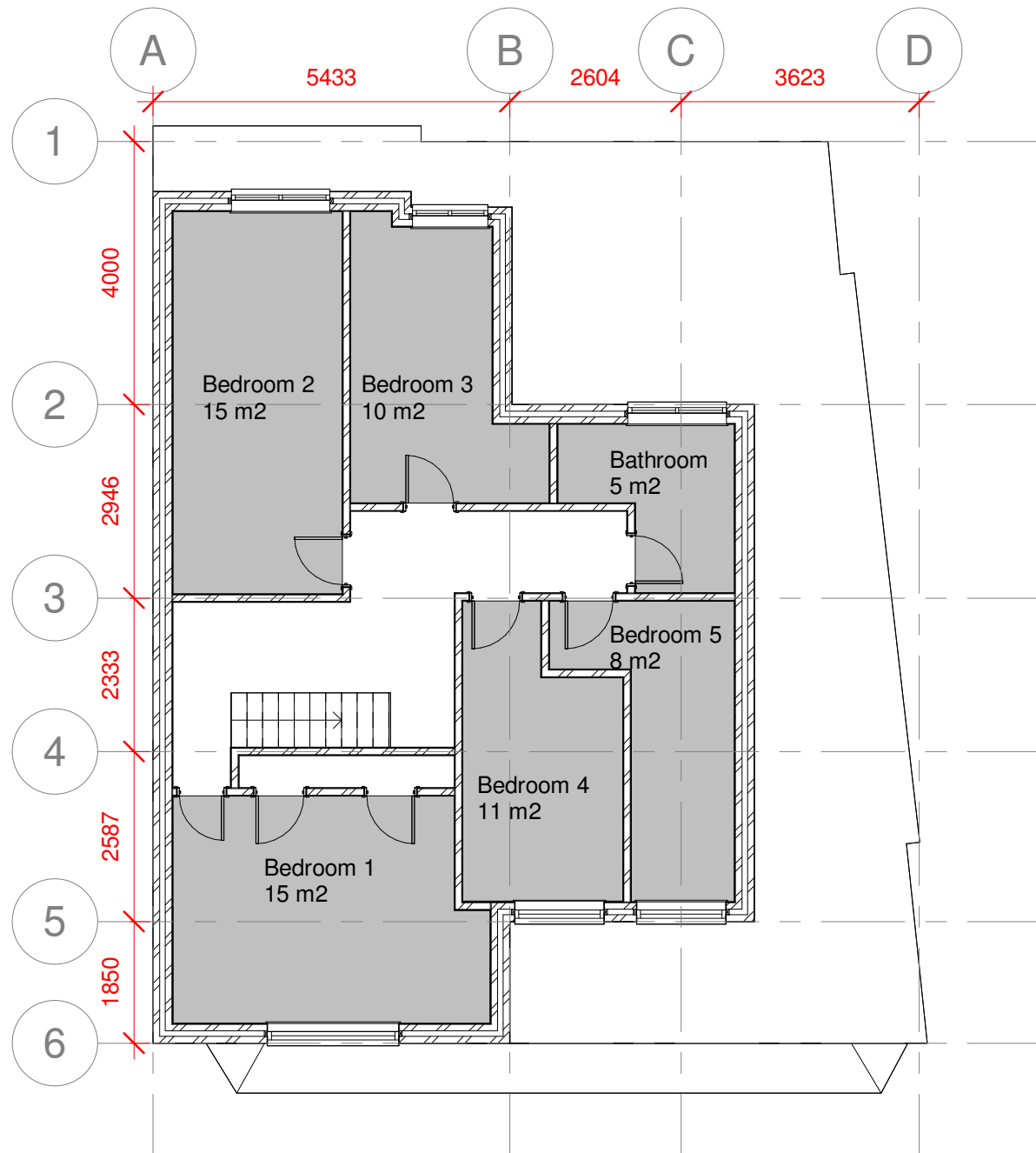
1 Existing First Floor Plan 1 : 100
