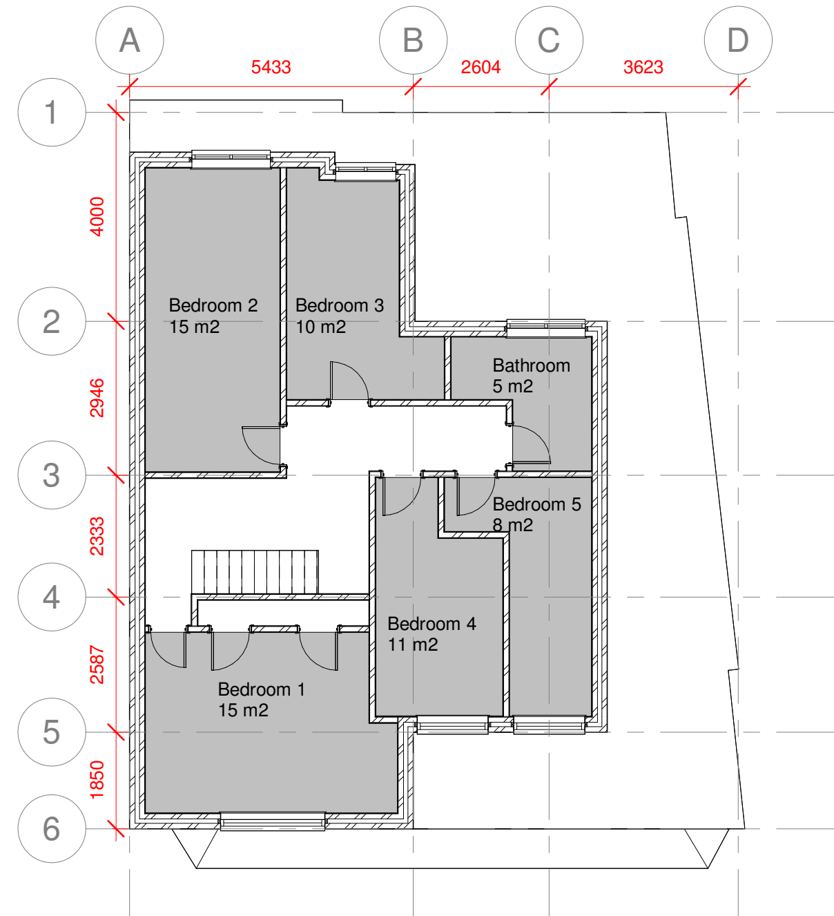
2 Proposed First Floor Plan 1 : 100
