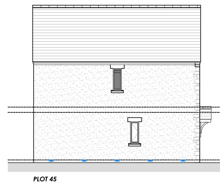
West Elevation
