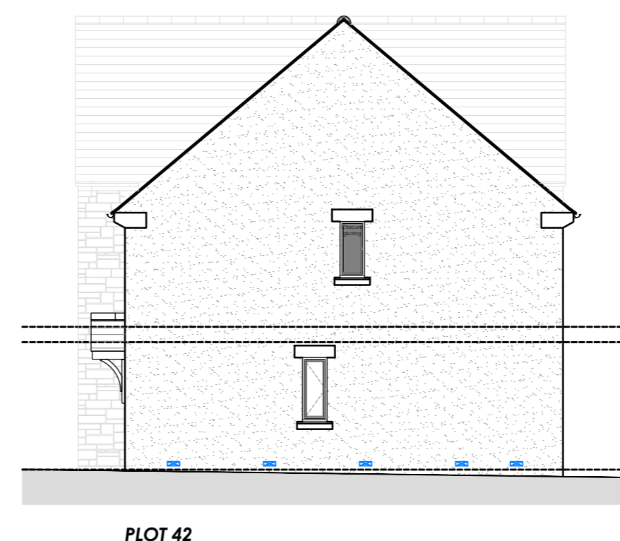
East Elevation
