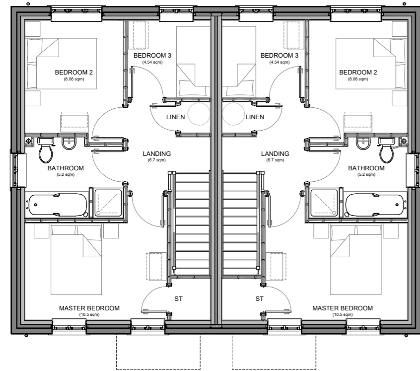
PLOT 52 PLOT 51 First Floor Plan
