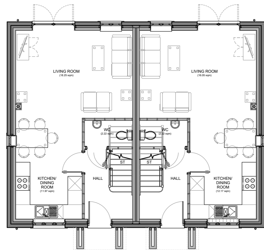
PLOT 52 PLOT 51 Ground Floor Plan
