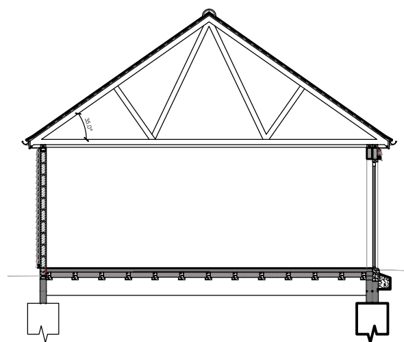
SECTION A
