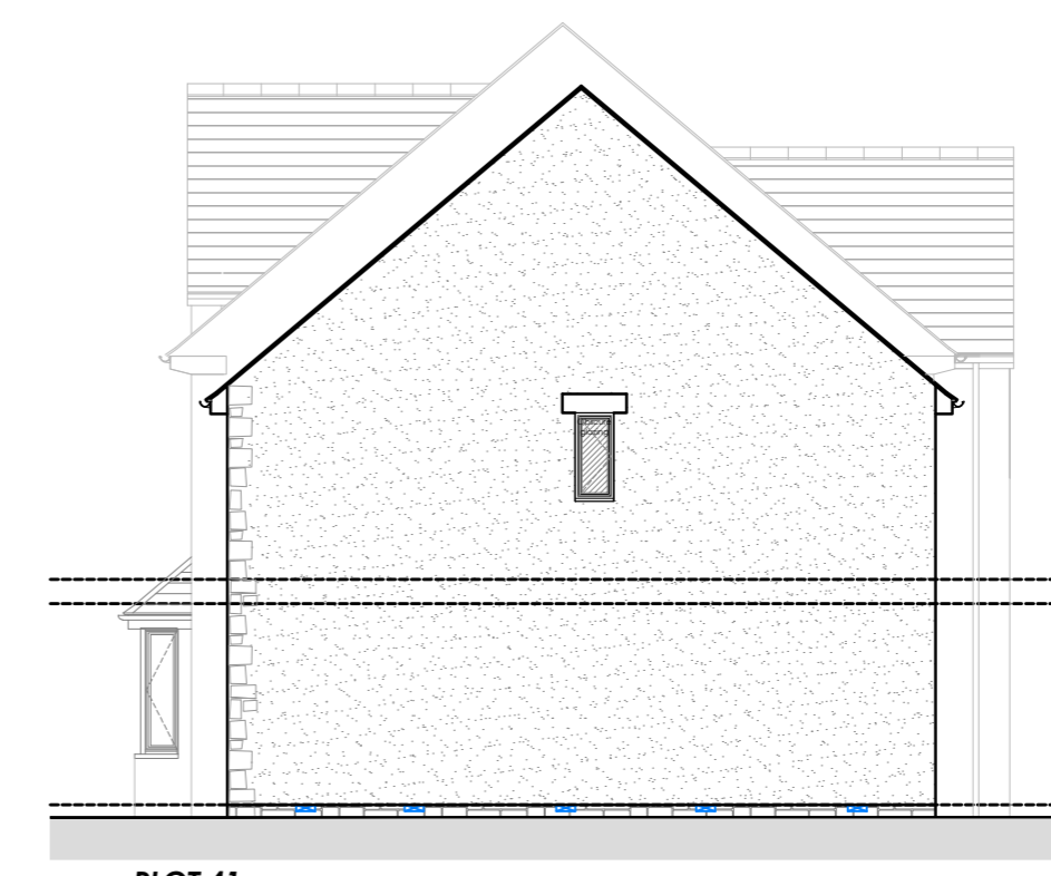
PLOT 41 West Elevation
