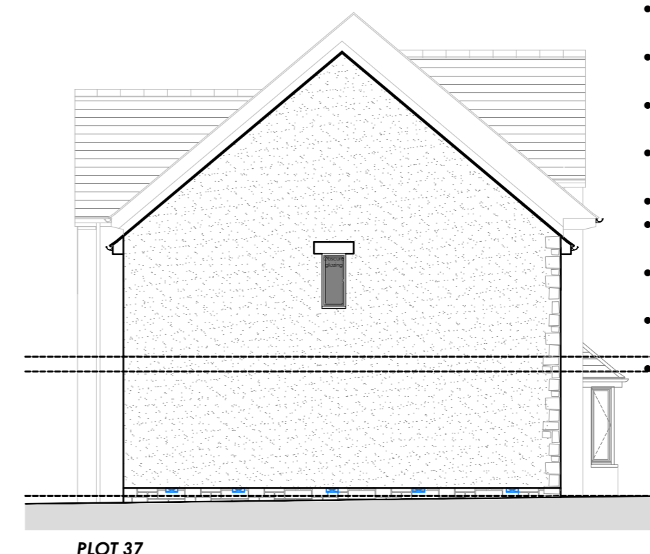
PLOT 37 East Elevation
