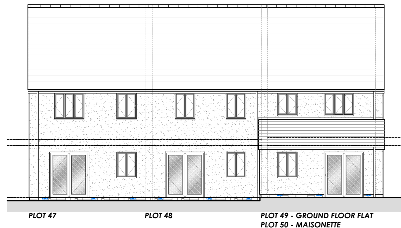
East Elevation
