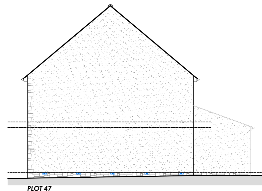
South Elevation
