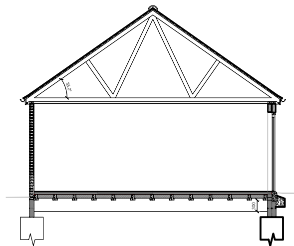
SECTION A
