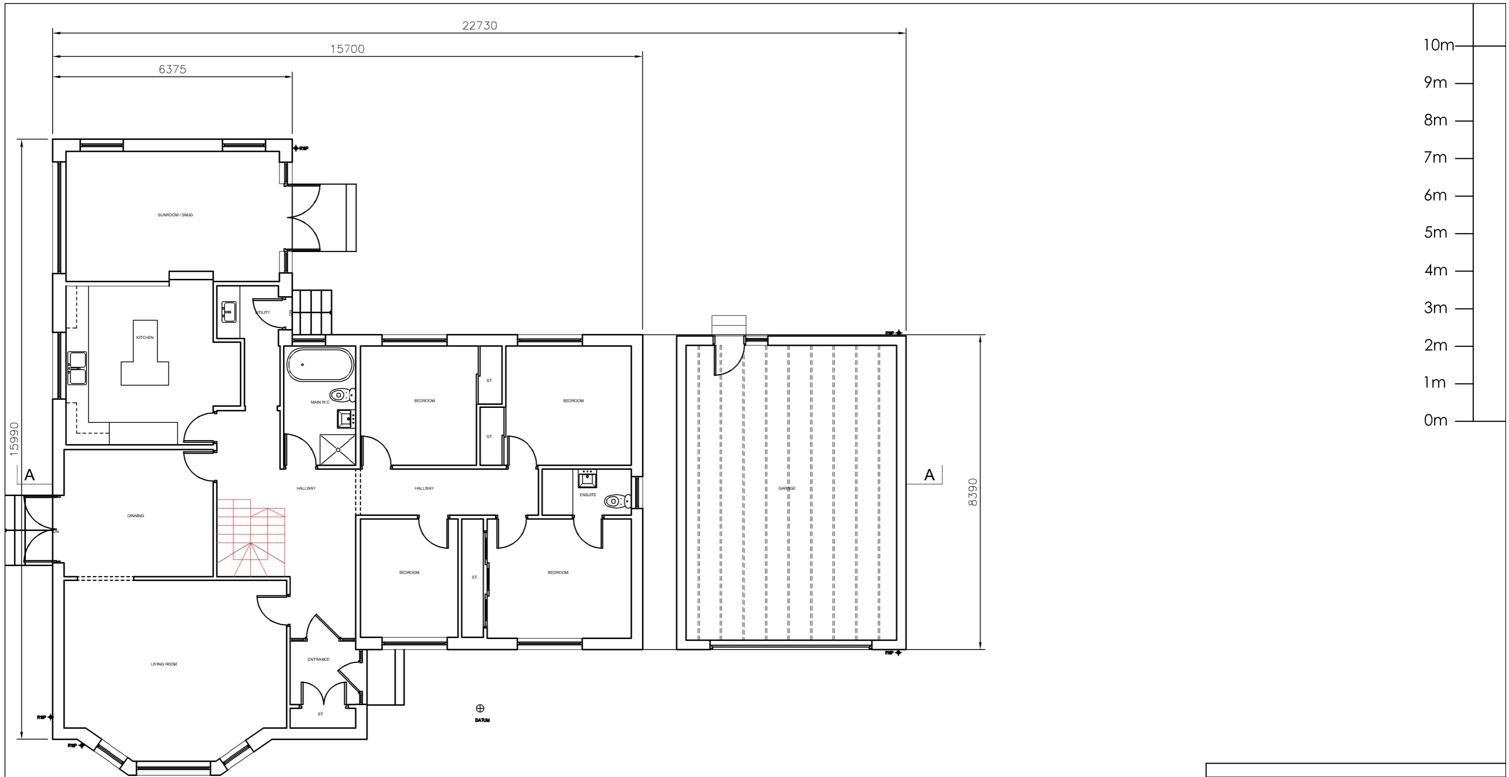
PROPOSED GROUND FLOOR PLAN 1:100 @ A3
