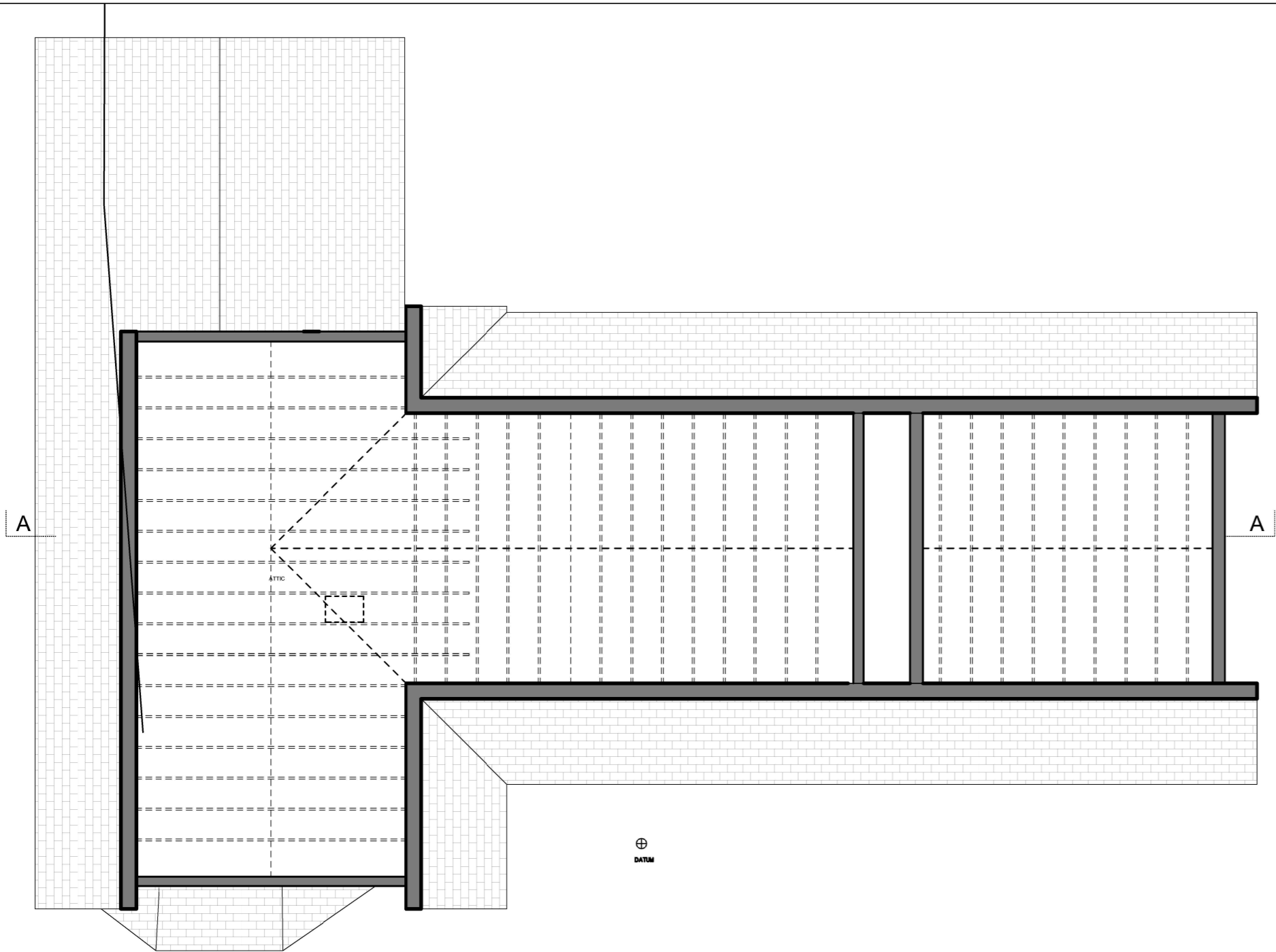
EXISTING ATTIC FLOOR PLAN 1:100 @ A3
