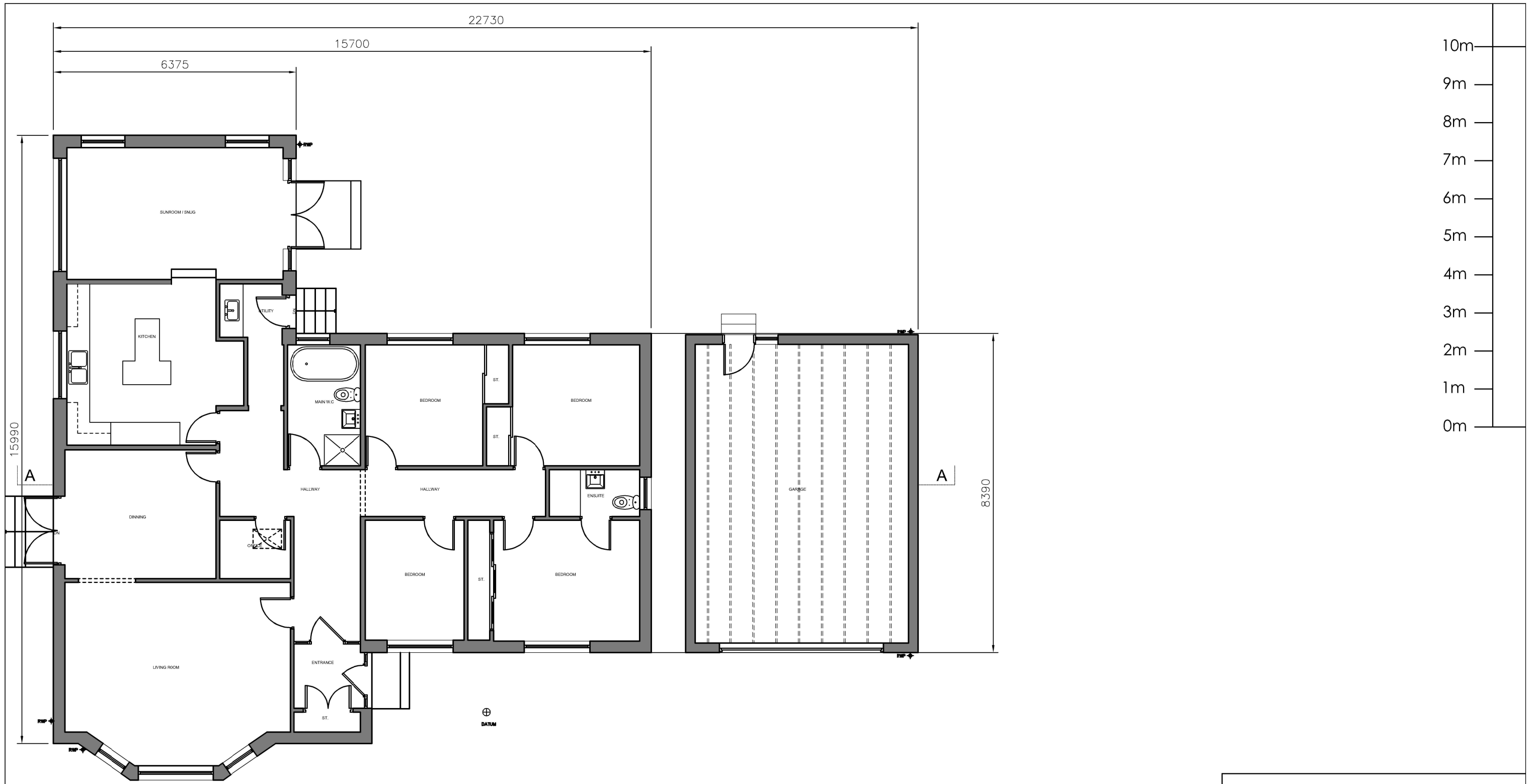
EXISTING GROUND FLOOR PLAN 1:100 @ A3
