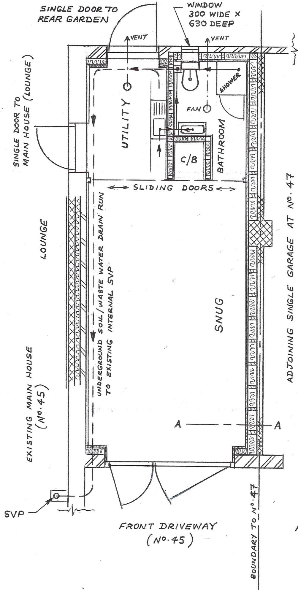
PROPOSED FLOOR PLAN - CONVERTED GARAGE
