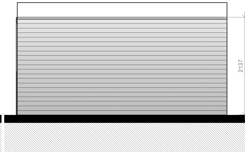
Rear Elevation 1 : 50
