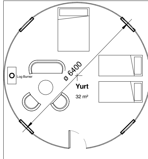
Ground Floor Plan 1 : 100
