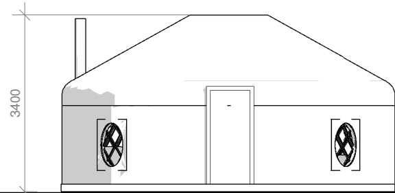
Front Elevation 1 : 100
