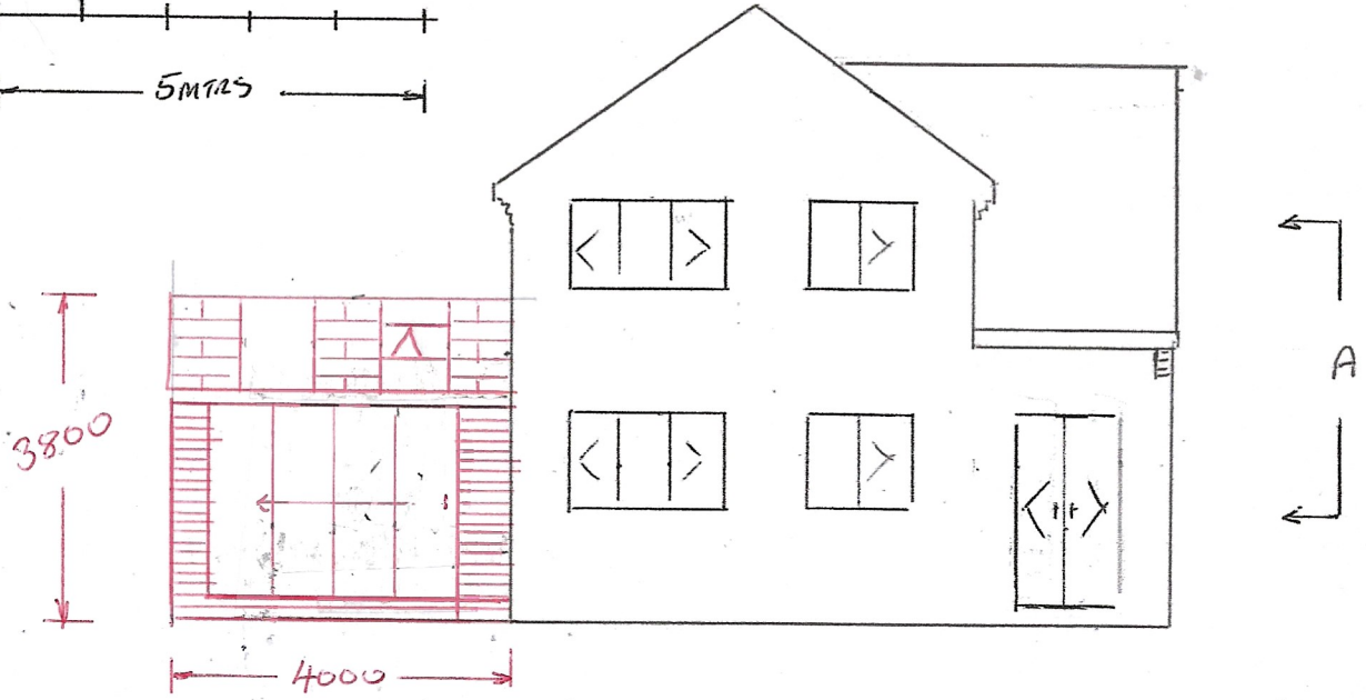
REAR ELEVATION
