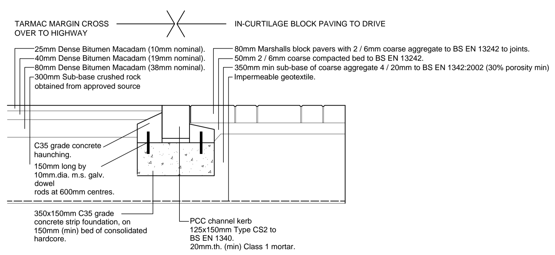
DETAIL SHOWING CONSTRUCTION OF TARMAC MARGIN/CROSS-OVER TO HIGHWAY AND JUNCTION TO BLOCK PAVING TO DRIVE. Scale 1:10
