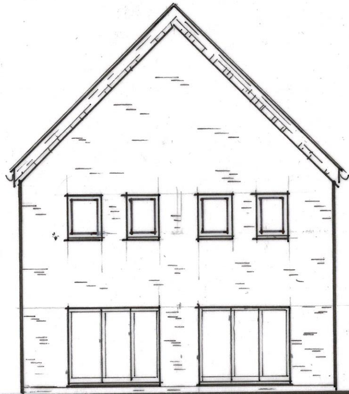
SOUTH WEST ELEVATION
