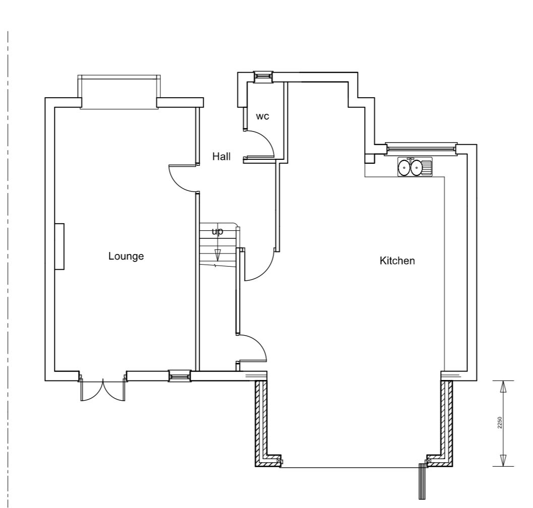
GROUND FLOOR (PROPOSED)
