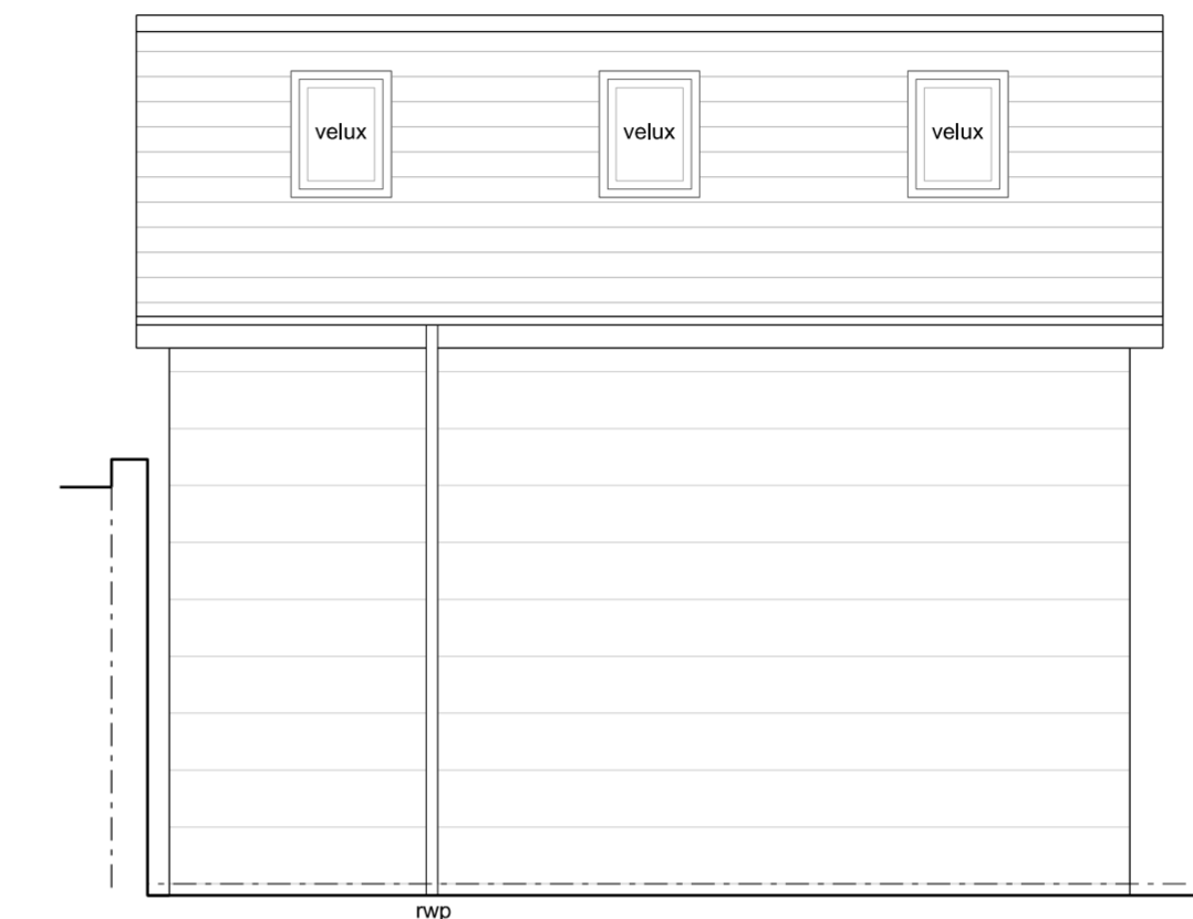
Proposed Front / West Elevation (facing Chapel Pitch. Existing trees / hedging omitted for clarity)
