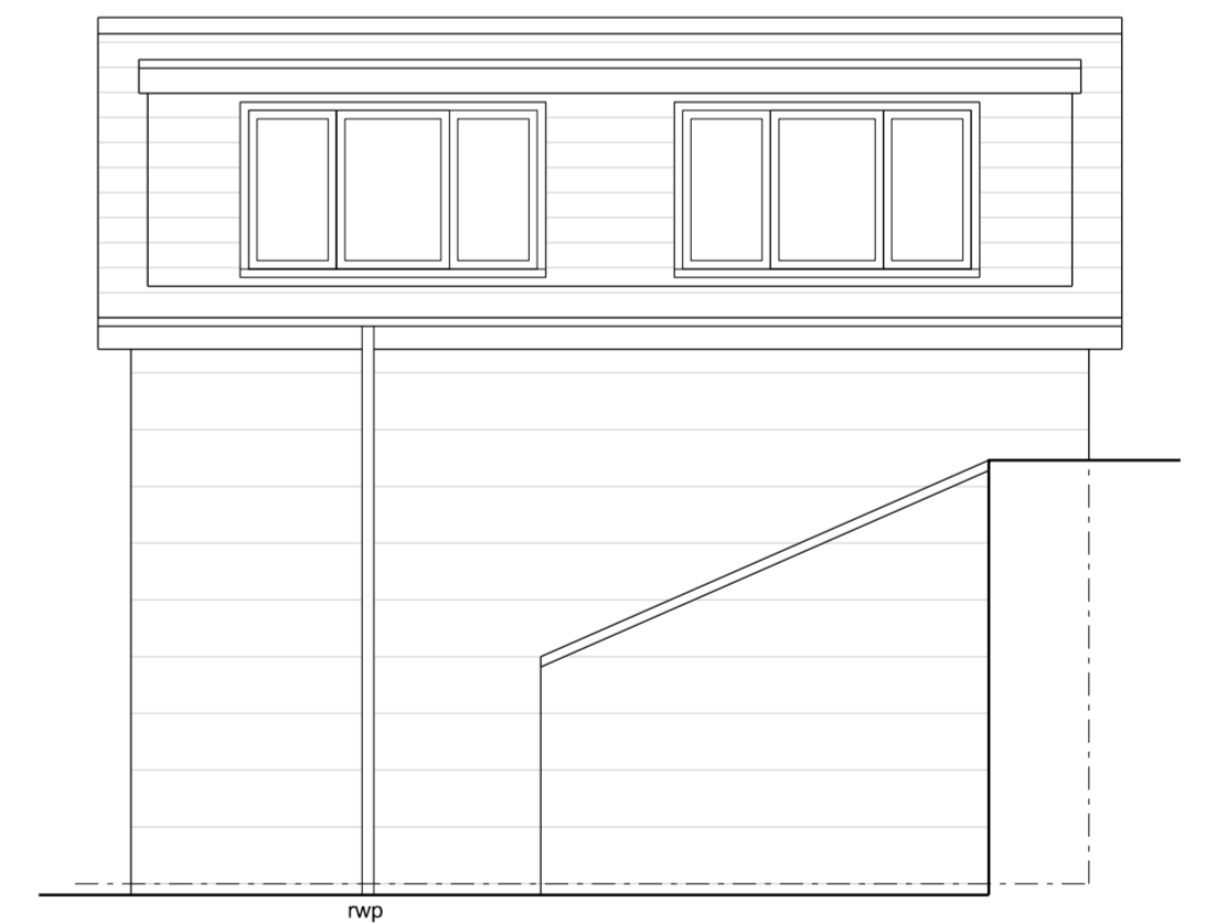
Proposed Rear / East Elevation (existing trees / hedging omitted for clarity)
