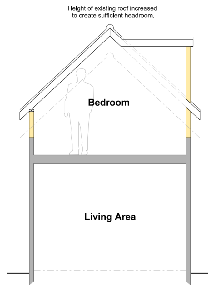
Proposed Section A-A
