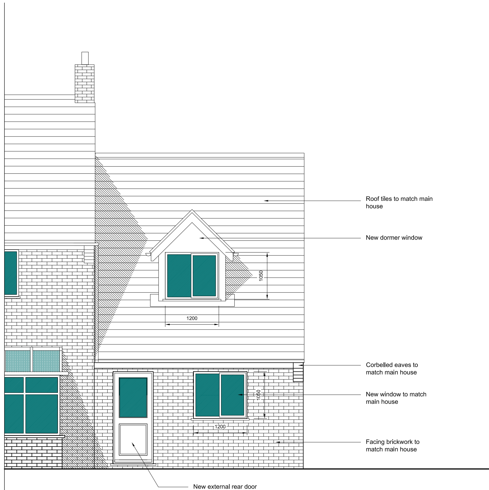
Proposed Rear Elevation Scale 1:50
