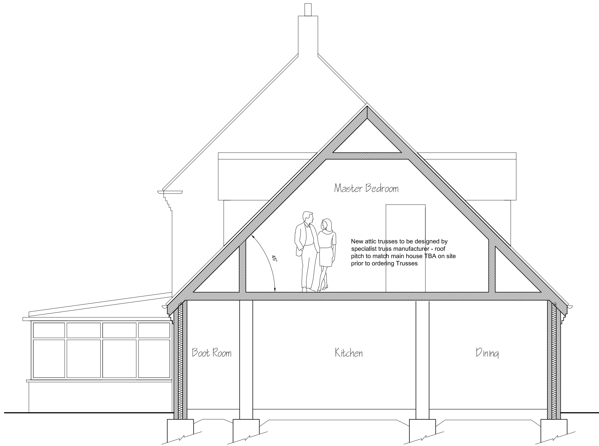
Proposed Section Thru' Scale 1:50
