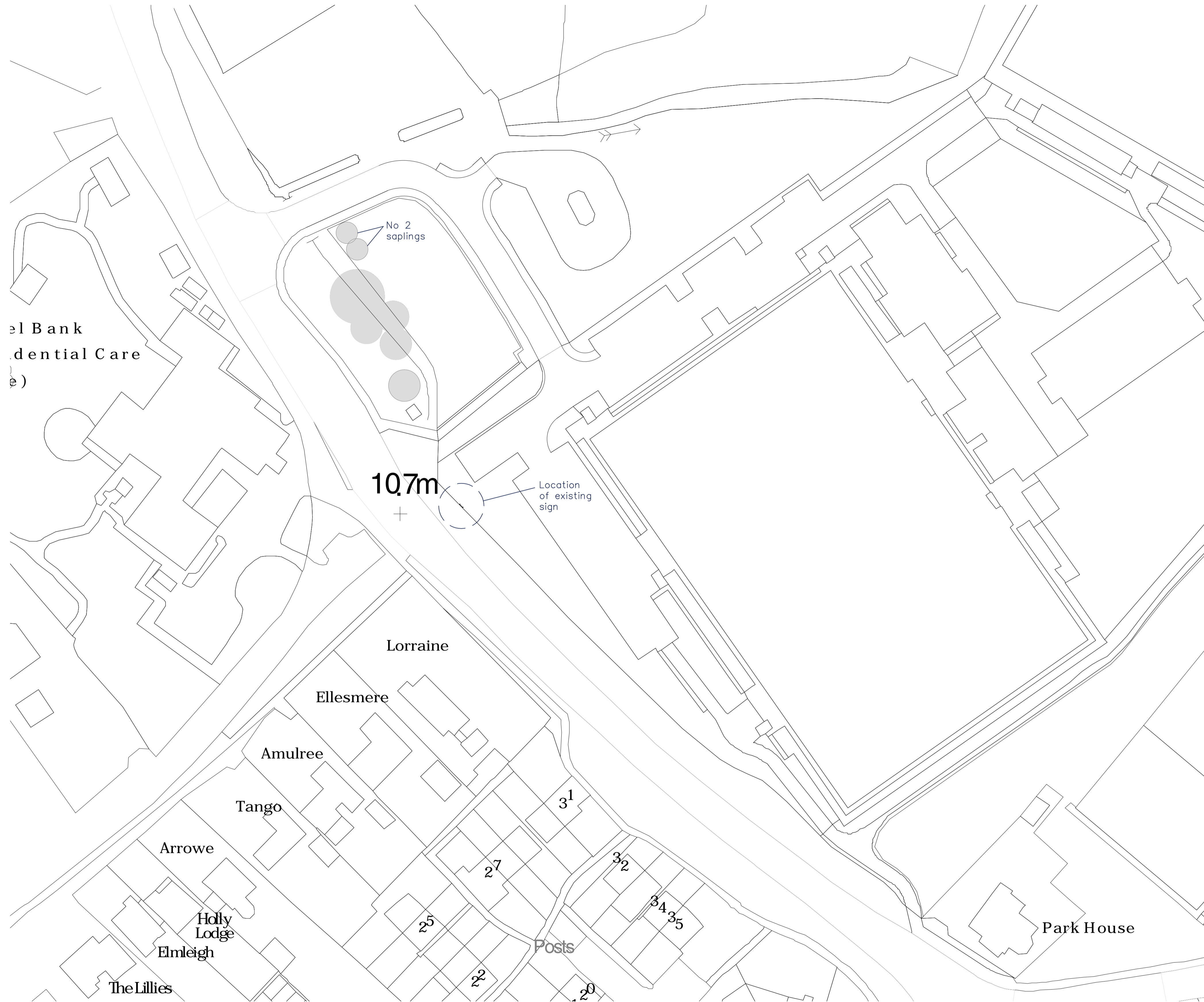
Site Plan AS EXISTING Scale 1:500
