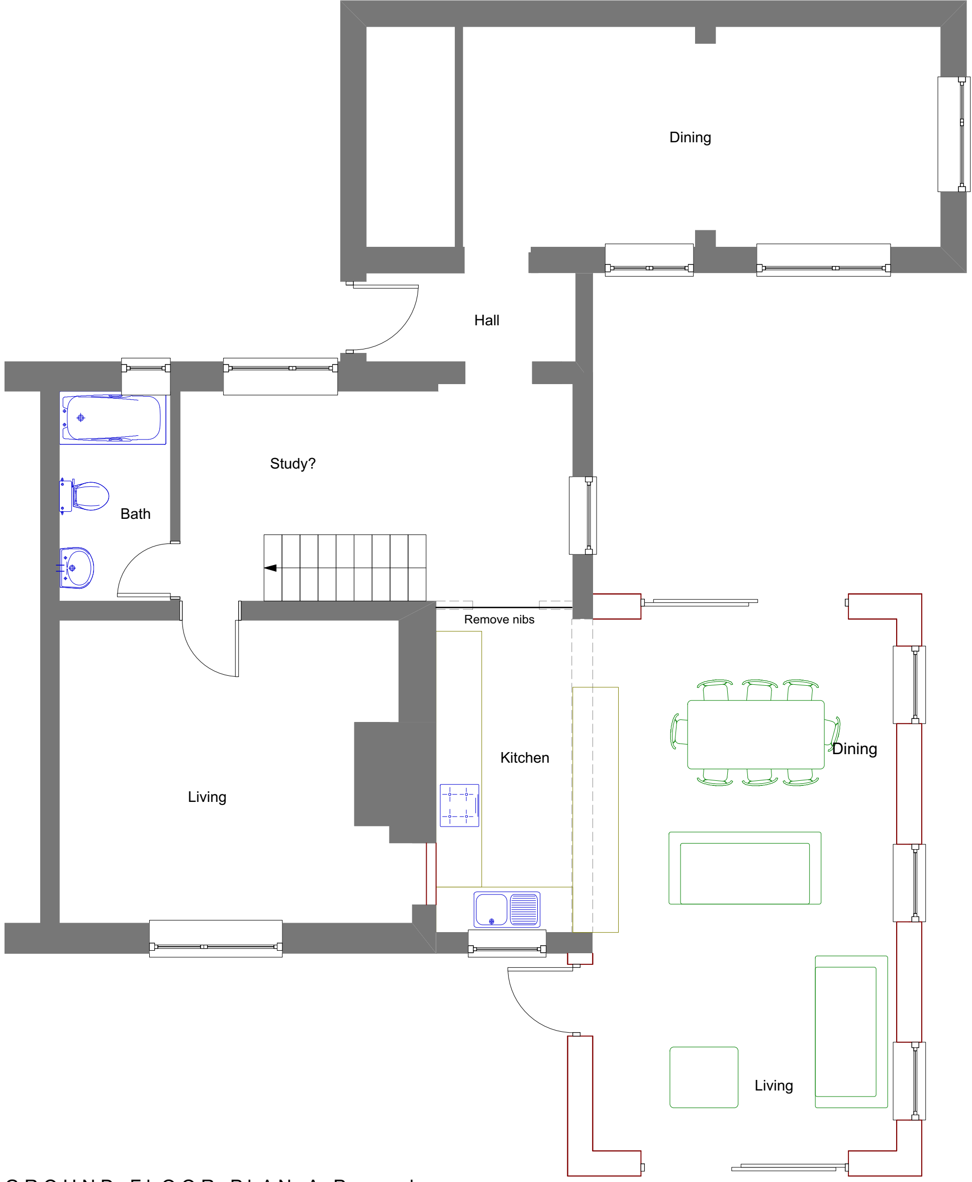
GROUND FLOOR PLAN As Proposed AT 1:50
