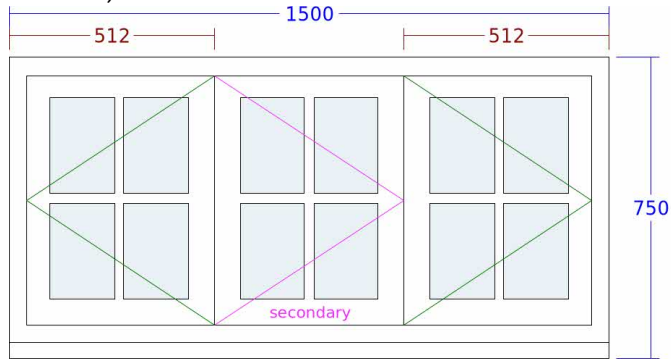
1. Conventional Cottage Window (Front elevation - First Floor W1)
