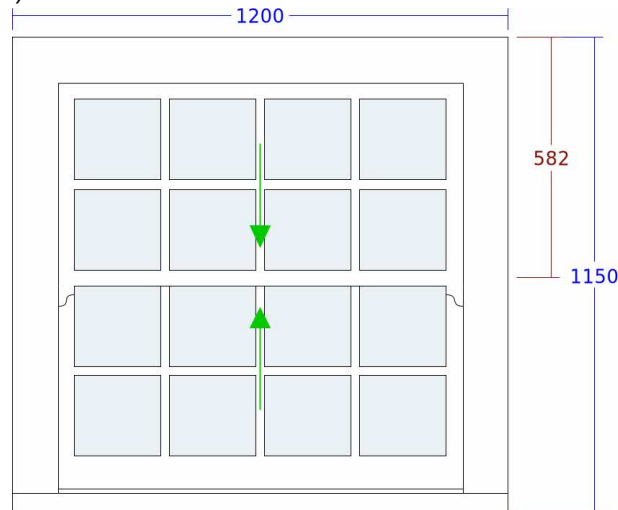
5. Sim Sash Window (Front elevation - Ground Floor Sash W1)
