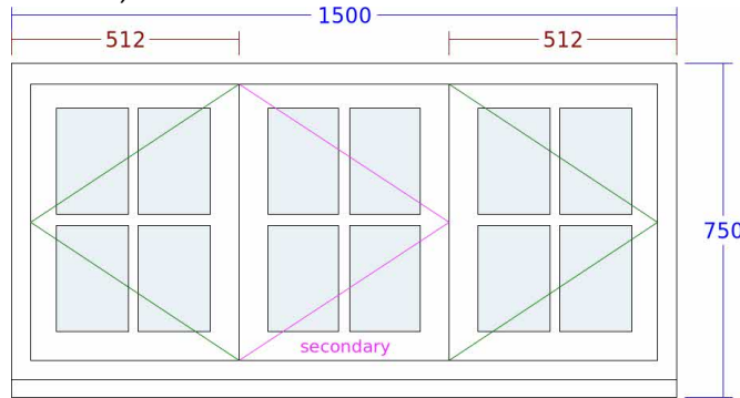
2. Conventional Cottage Window (Front elevation- First Floor W2)
