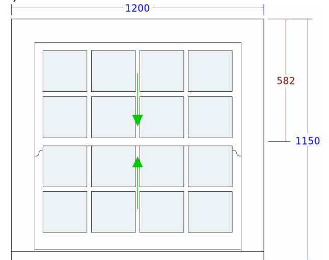
6. Sim Sash Window (Front elevation - Ground Floor Sash W2)
