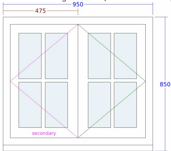
4. Conventional Cottage Window (Side elevation - W2)
