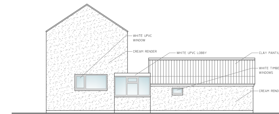
SIDE ELEVATION 1:100 - WEST
