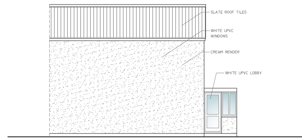
REAR ELEVATION 1:100 - NORTH
