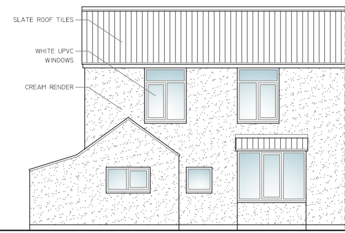
FRONT ELEVATION 1:100 - SOUTH
