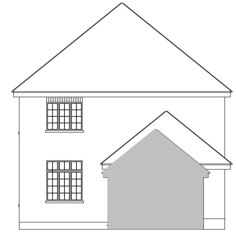
East Elevation Proposed
