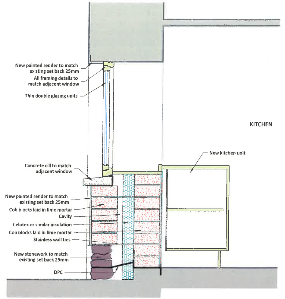
CROSS SECTION THROUGH NEW WINDOW AS PROPOSED 1:20
