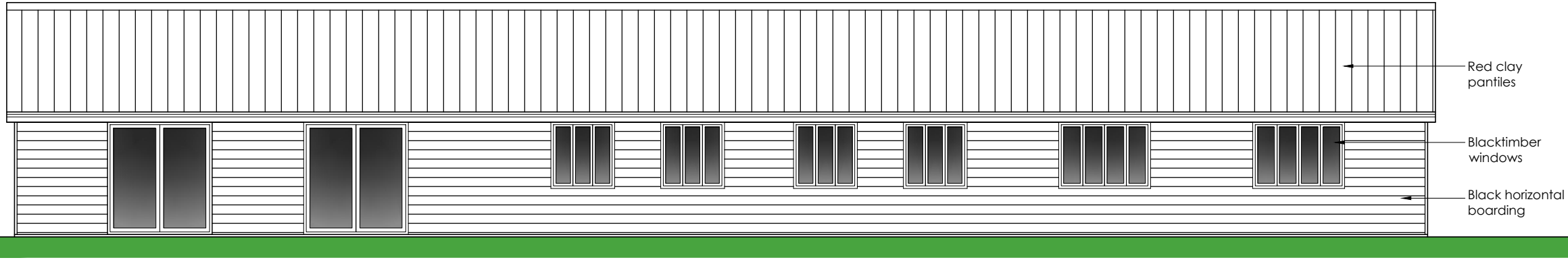
EXISTING SIDE ELEVATION - WEST
