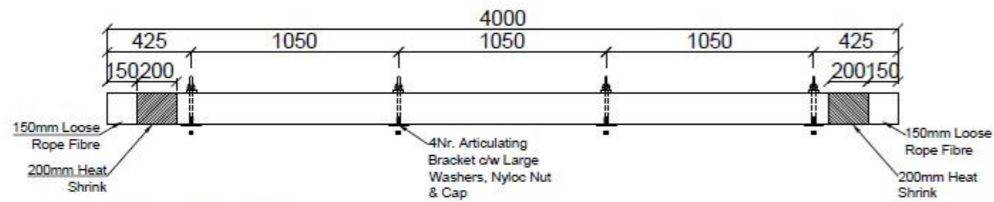
Cat Rope Cut to Size
