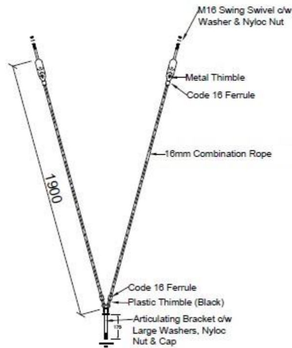
Cat Rope Suspension Rope Detail
