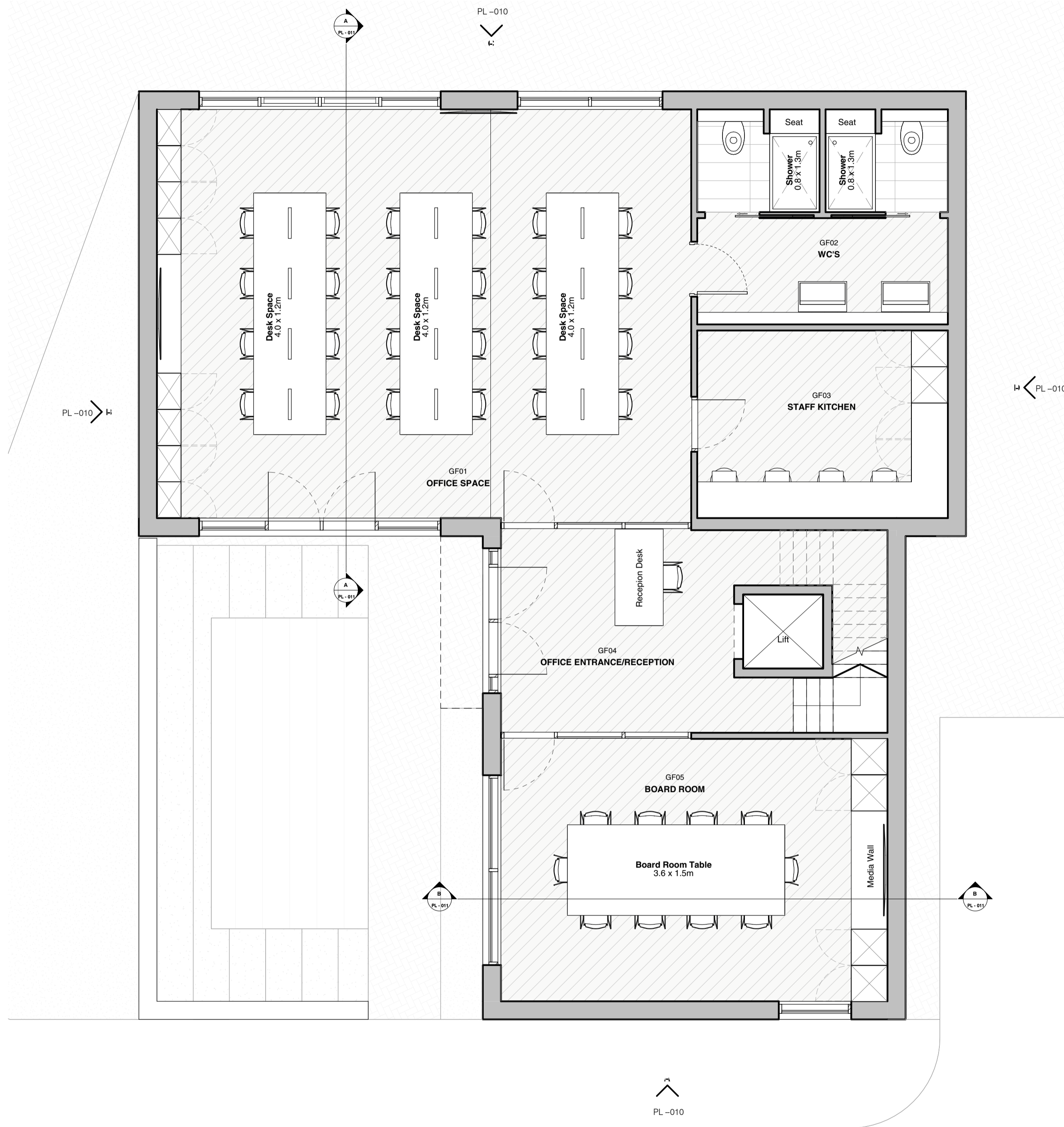
UNIT 01 - PROPOSED GROUND FLOOR PLAN 1 : 50
