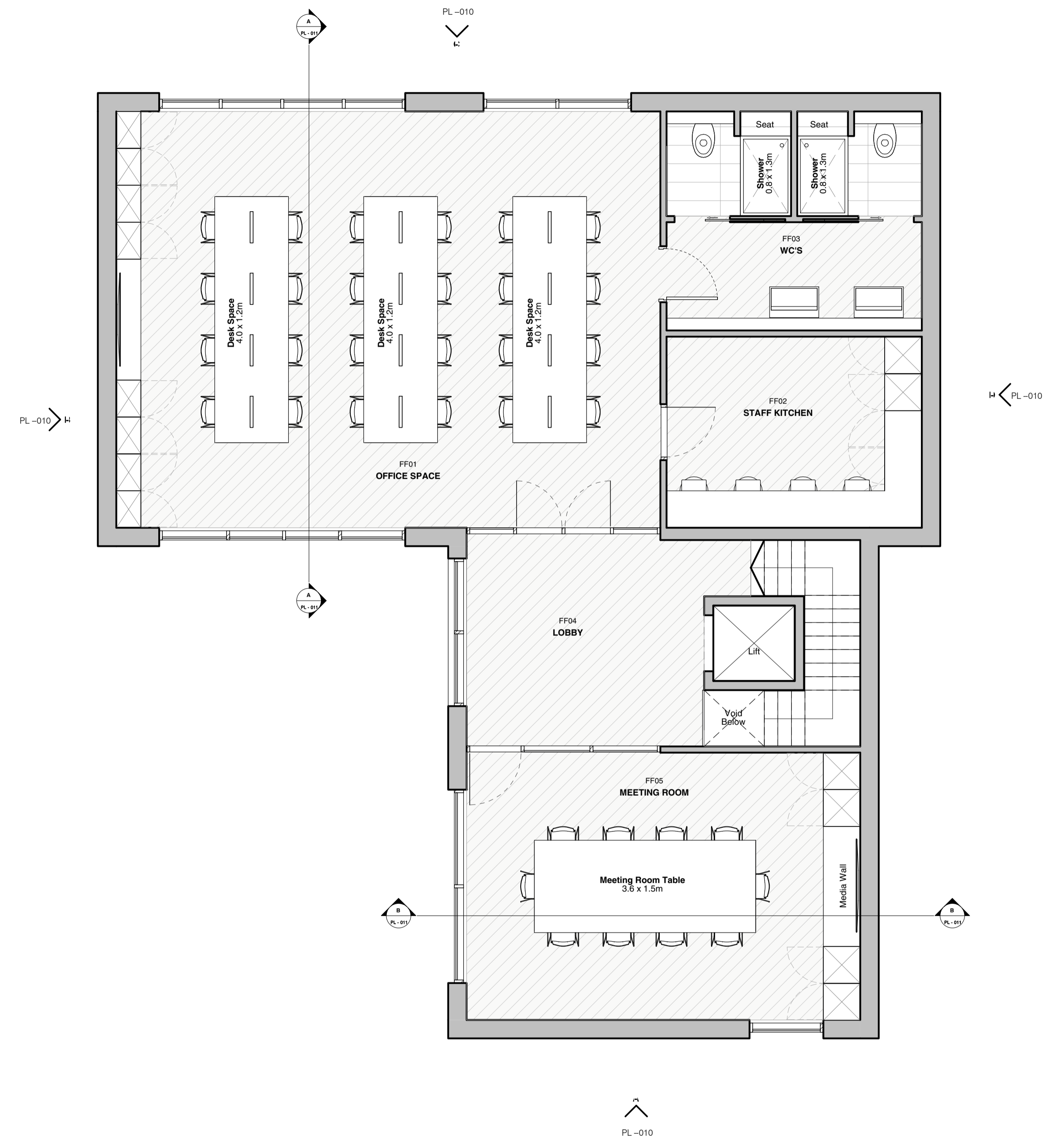
UNIT 01 - PROPOSED FIRST FLOOR PLAN 1 : 50
