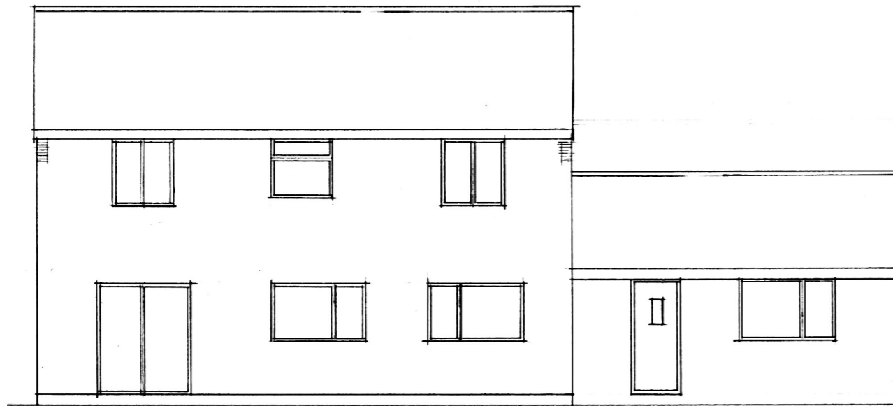
REAR ELEVATION
