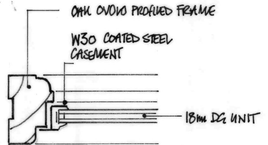
window head • jamb SOLID EUROPEAN OAK
