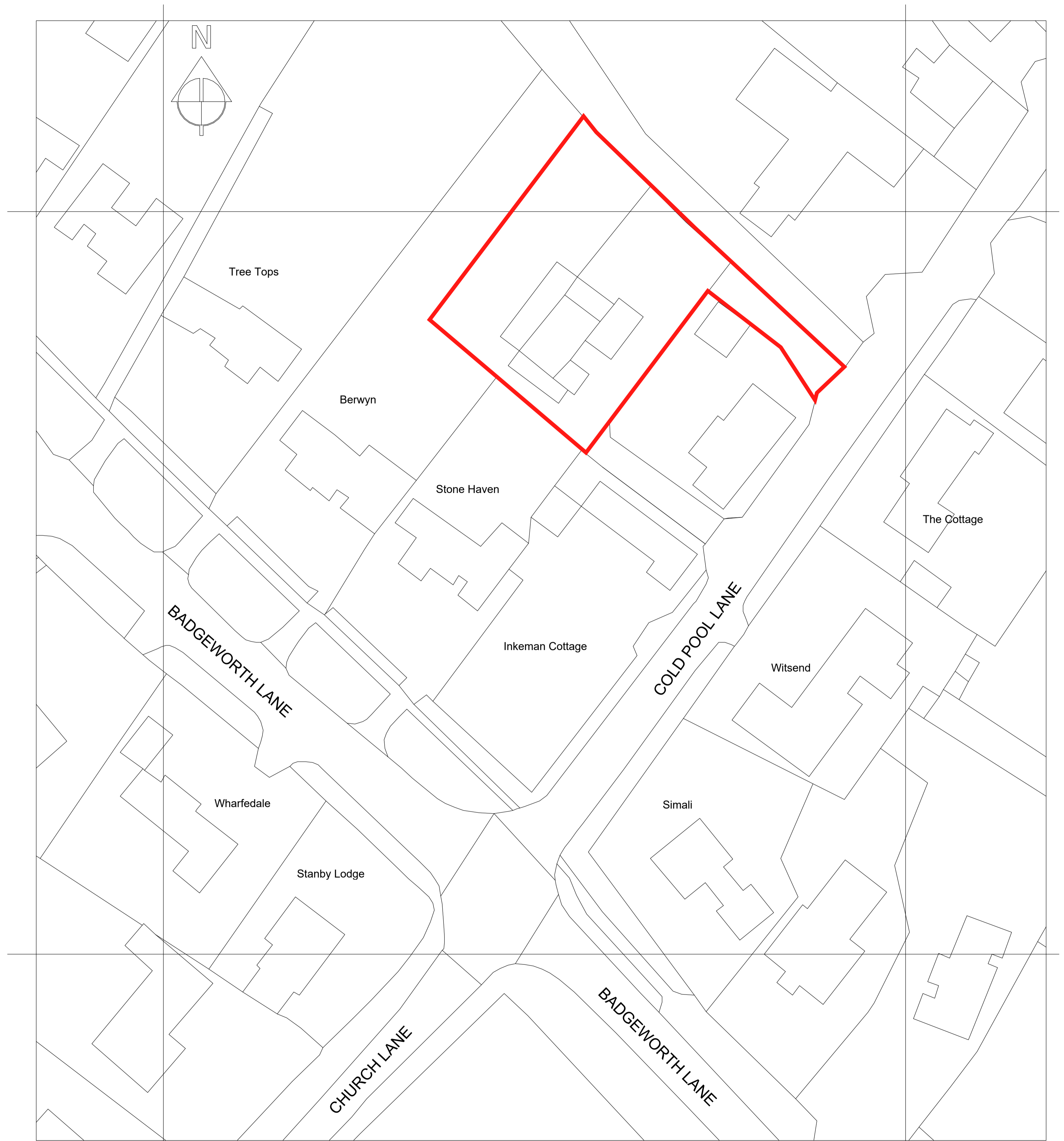
EXISTING SITE LOCATION SCALE: 1:300 @ A1
