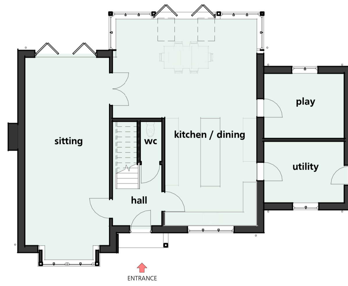
ground floor 1 : 100
