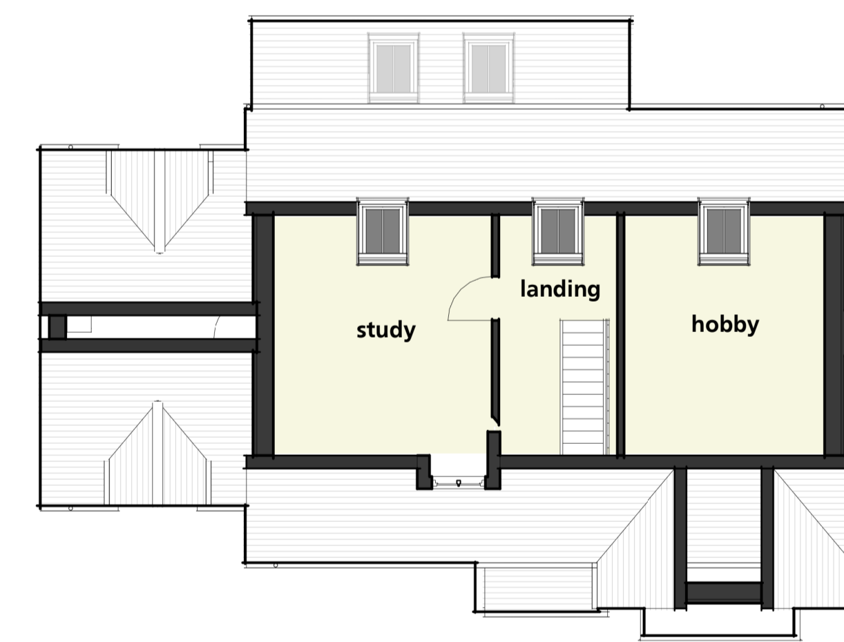
second floor 1 : 100
