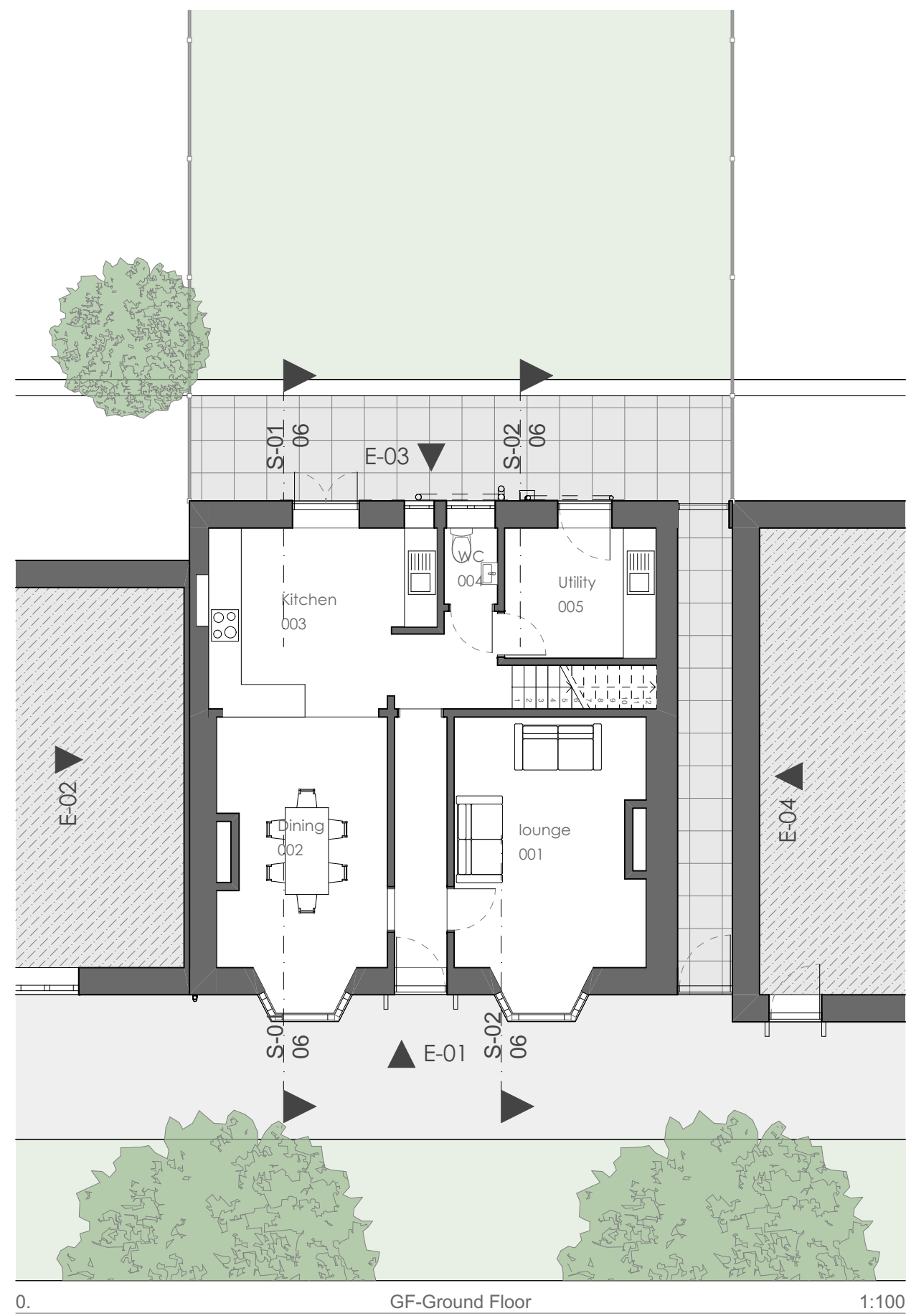
0. GF-Ground Floor 1:100
