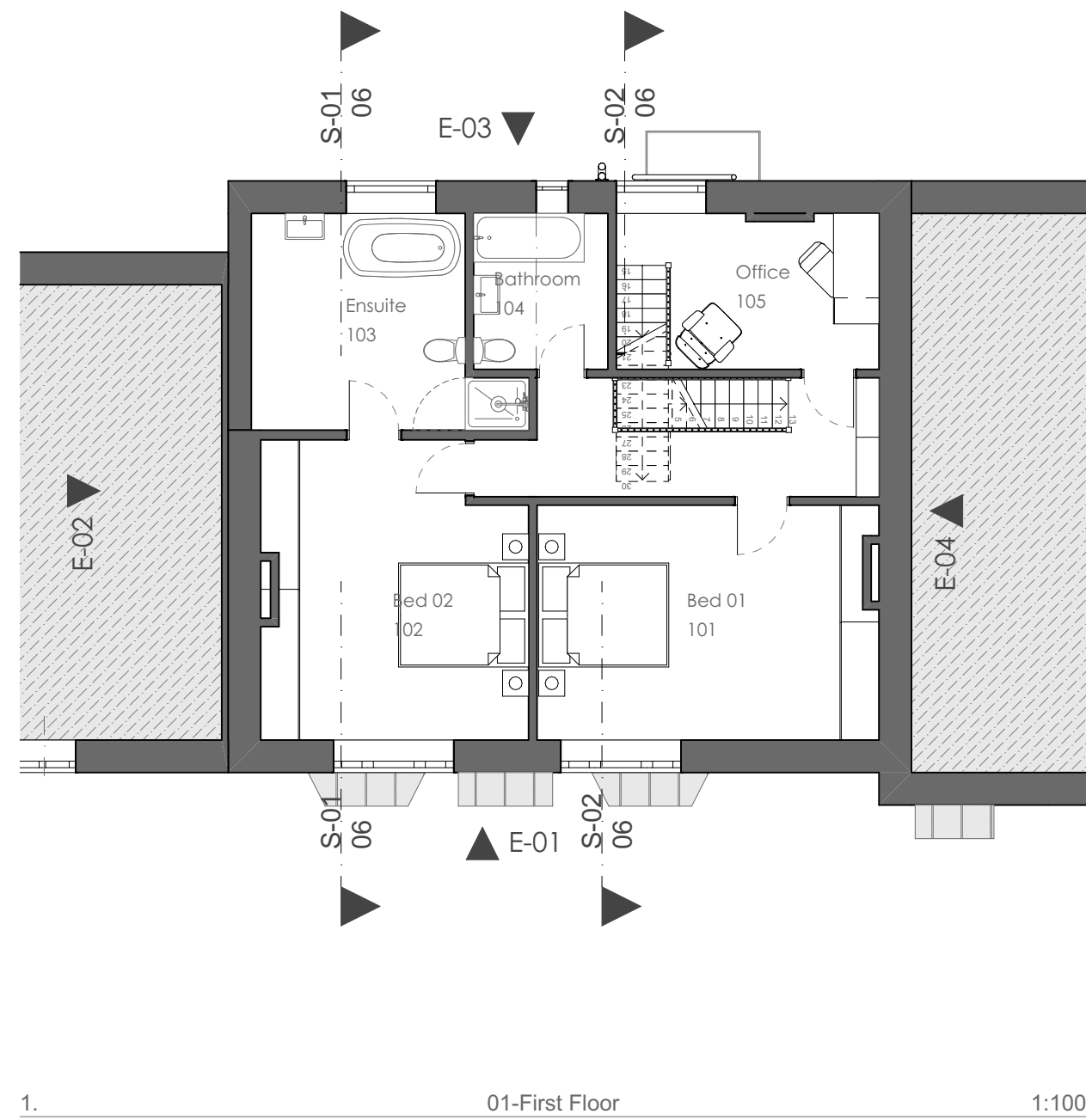
1. 01-First Floor 1:100
