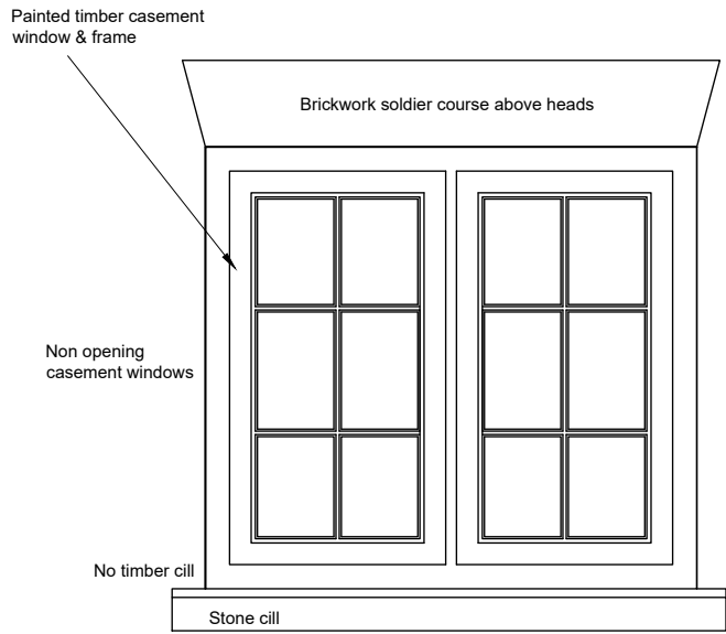
EXISTING WINDOW ELEVATION (single glazed)
