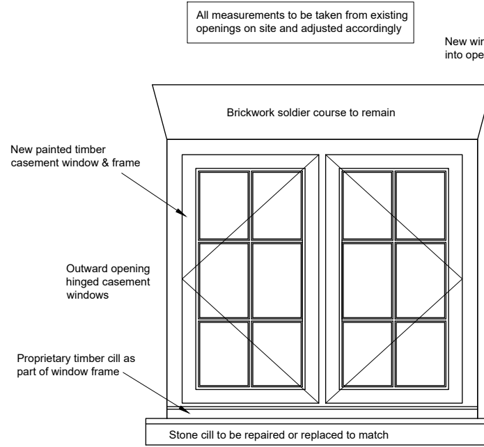
PROPOSED WINDOW ELEVATION (single glazed)
