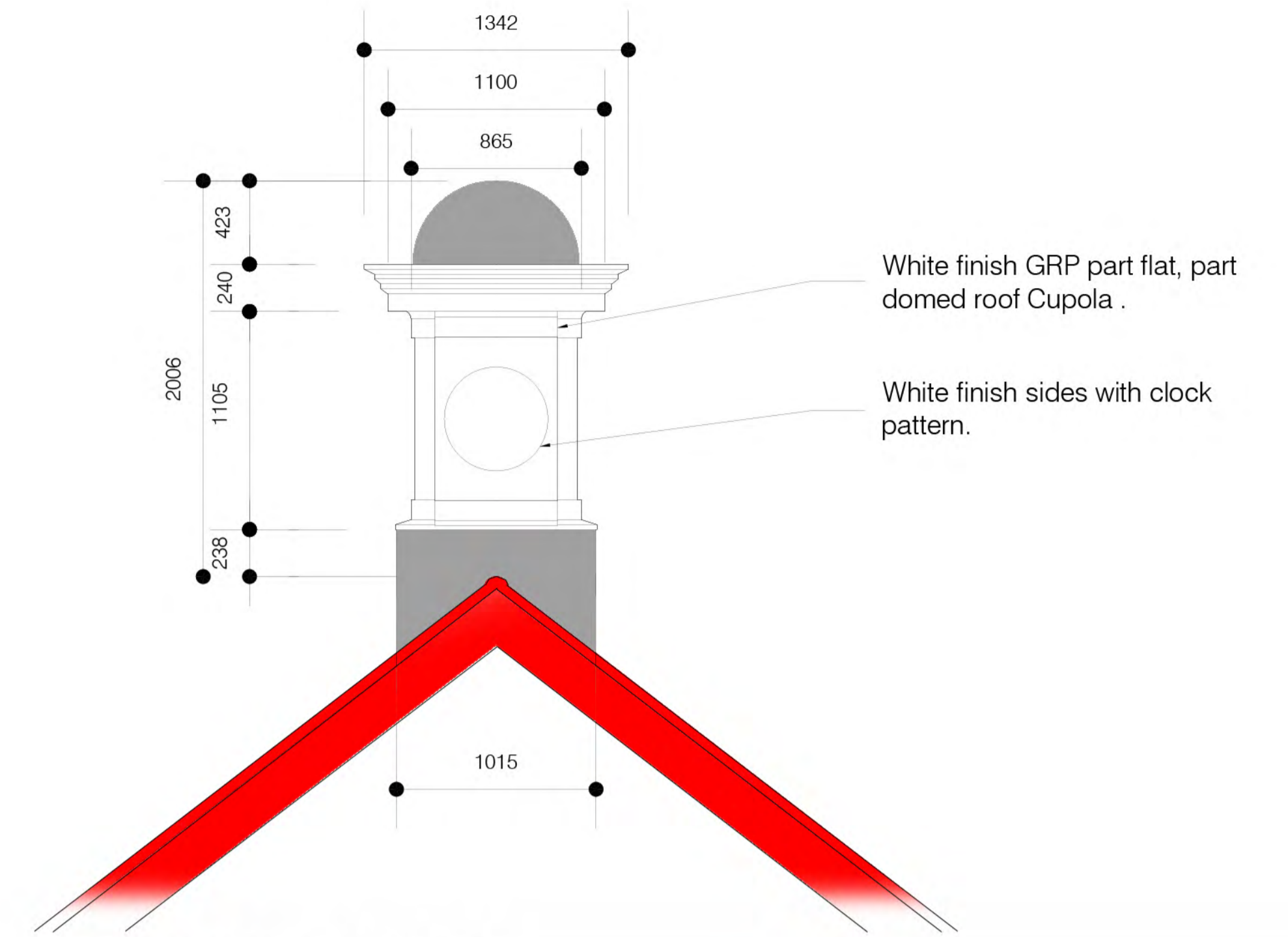
Proposed Cupola Detail 1:50
