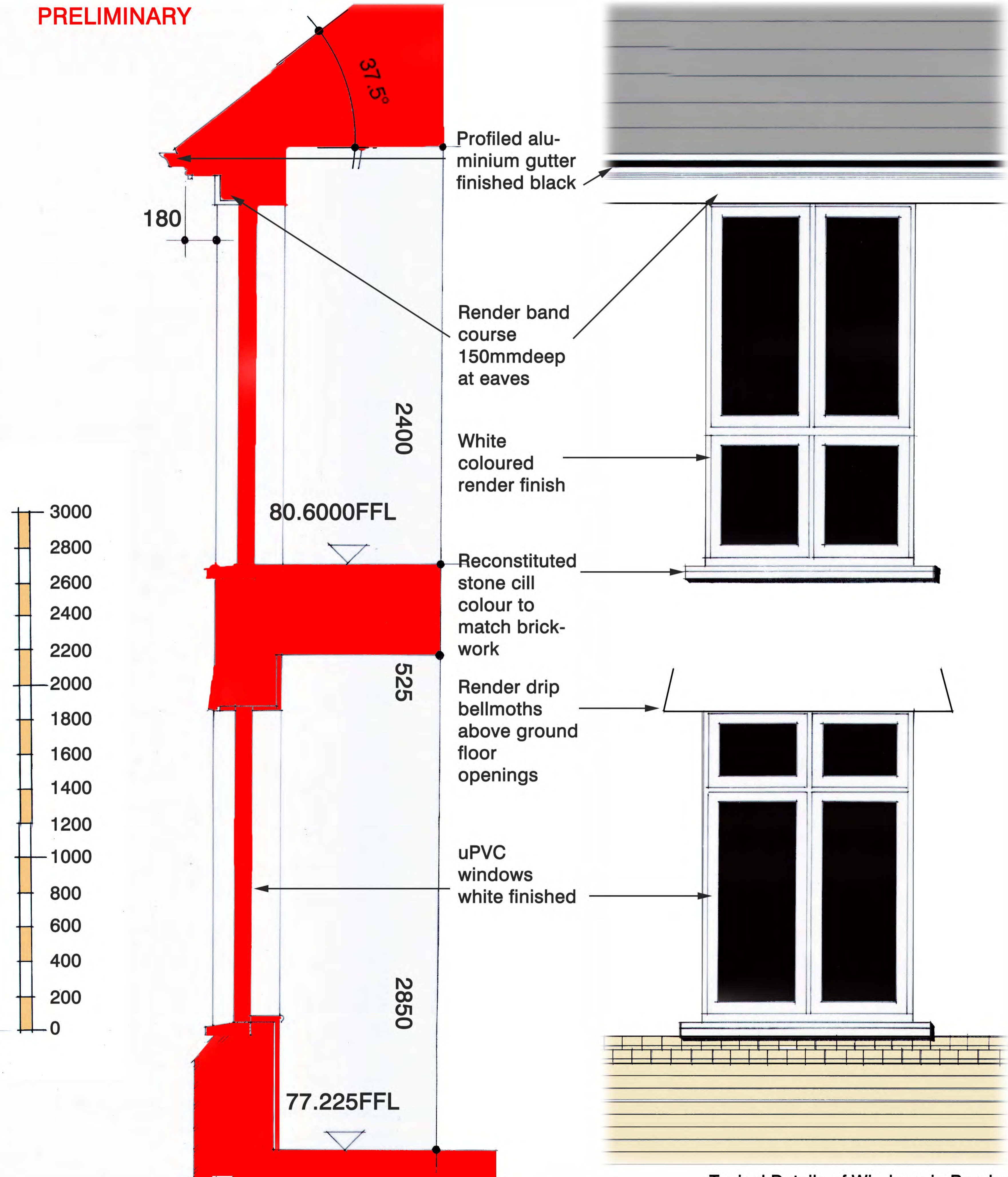
Typical Details of Windows in Render 1:25
