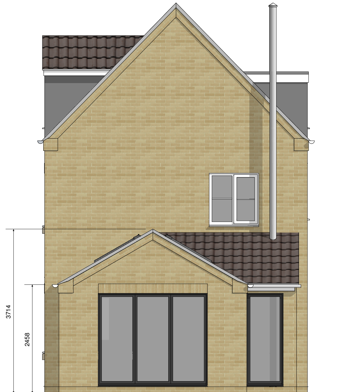
Proposed West Elevation
