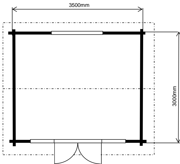
Proposed Garden Room - 1 Pikes Hill - SO43 7AS
