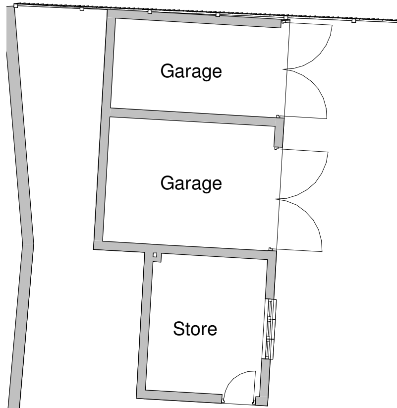
5 Garage Ground Floor 1 : 100
