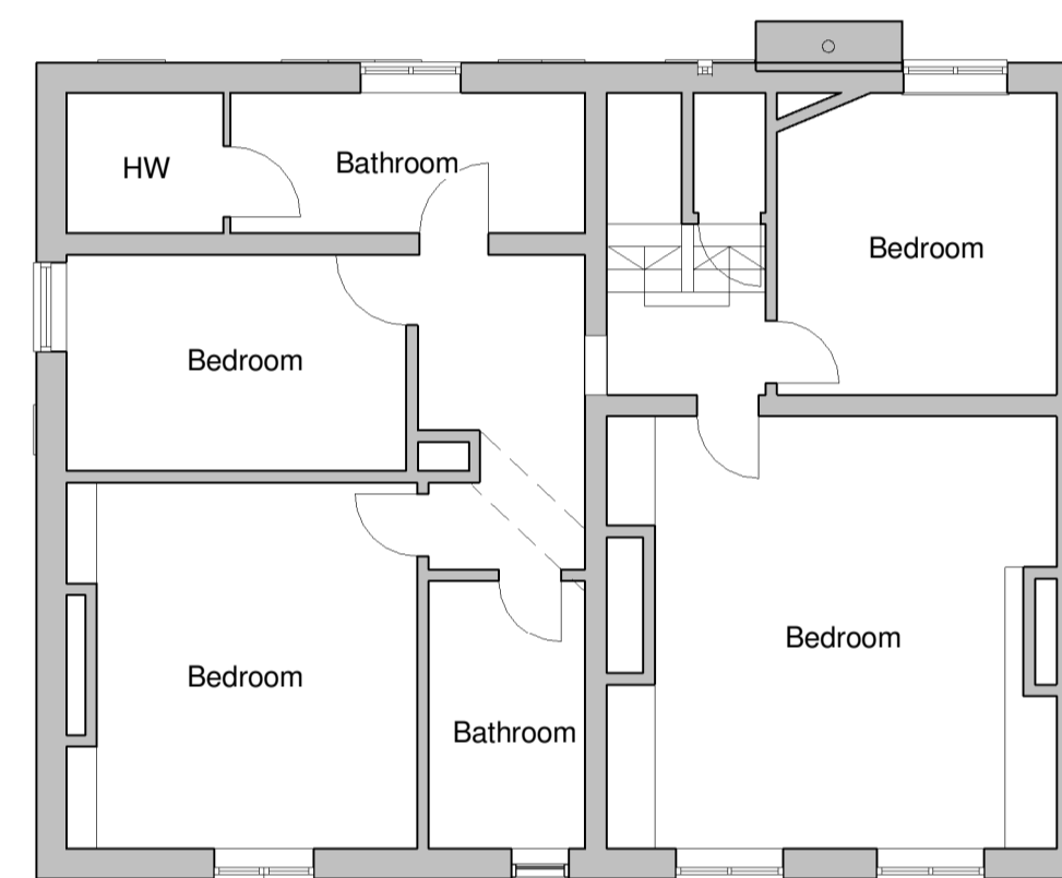
3 20 First Floor 1 : 100
