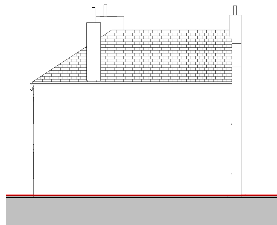
5 North Elevation 1 : 100
