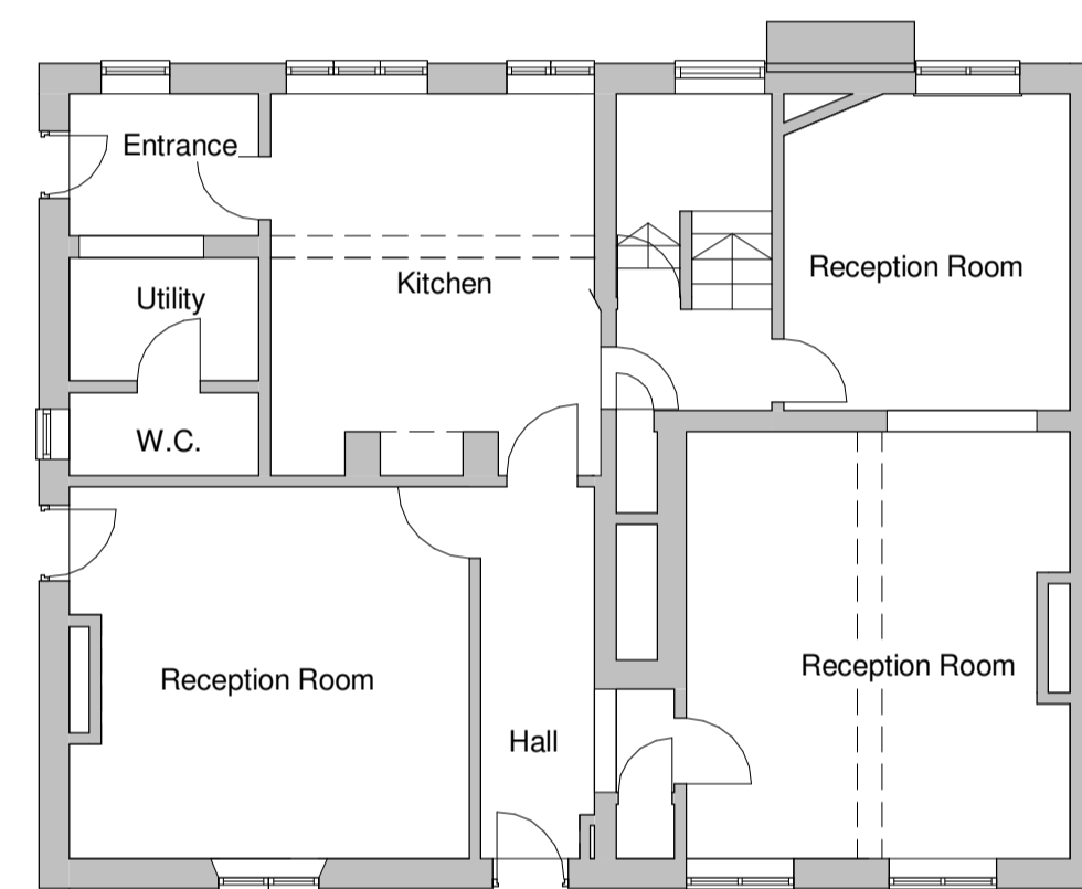
1 10 Ground Floor 1 : 100
